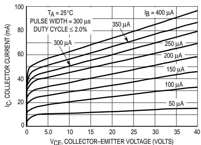
Figure 7. Collector Characteristics
