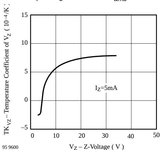
Figure 3. Temperature Coefficient of V_Z vs. Z-Voltage
