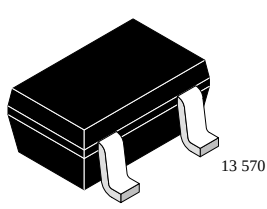
BFS17AW Marking: WE2 Plastic case (SOT 323) 1 = Collector, 2 = Base, 3 = Emitter
