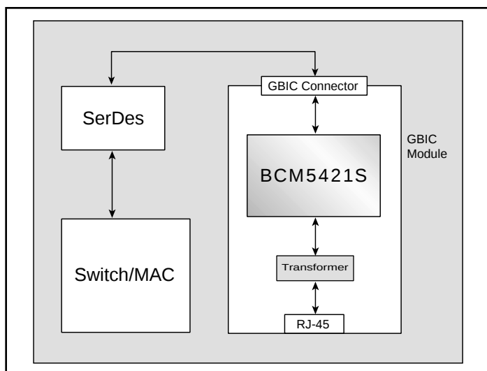
10/100/1000BASE-T GBIC Module
