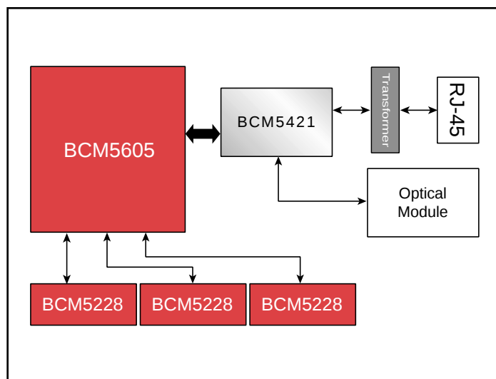
1000BASE-T Gigabit Copper or Fiber Uplink
