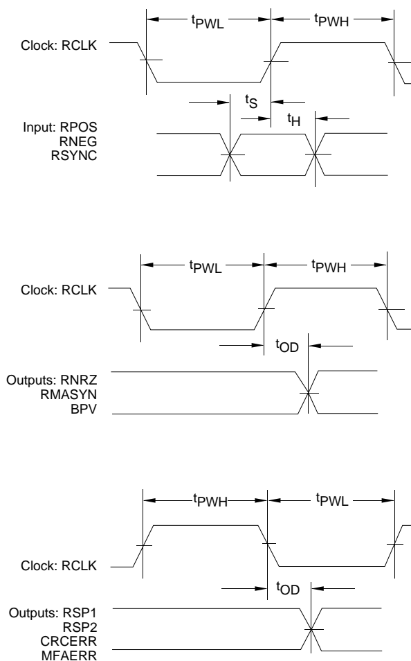
Figure 13. RCLK Input/Output Timing
