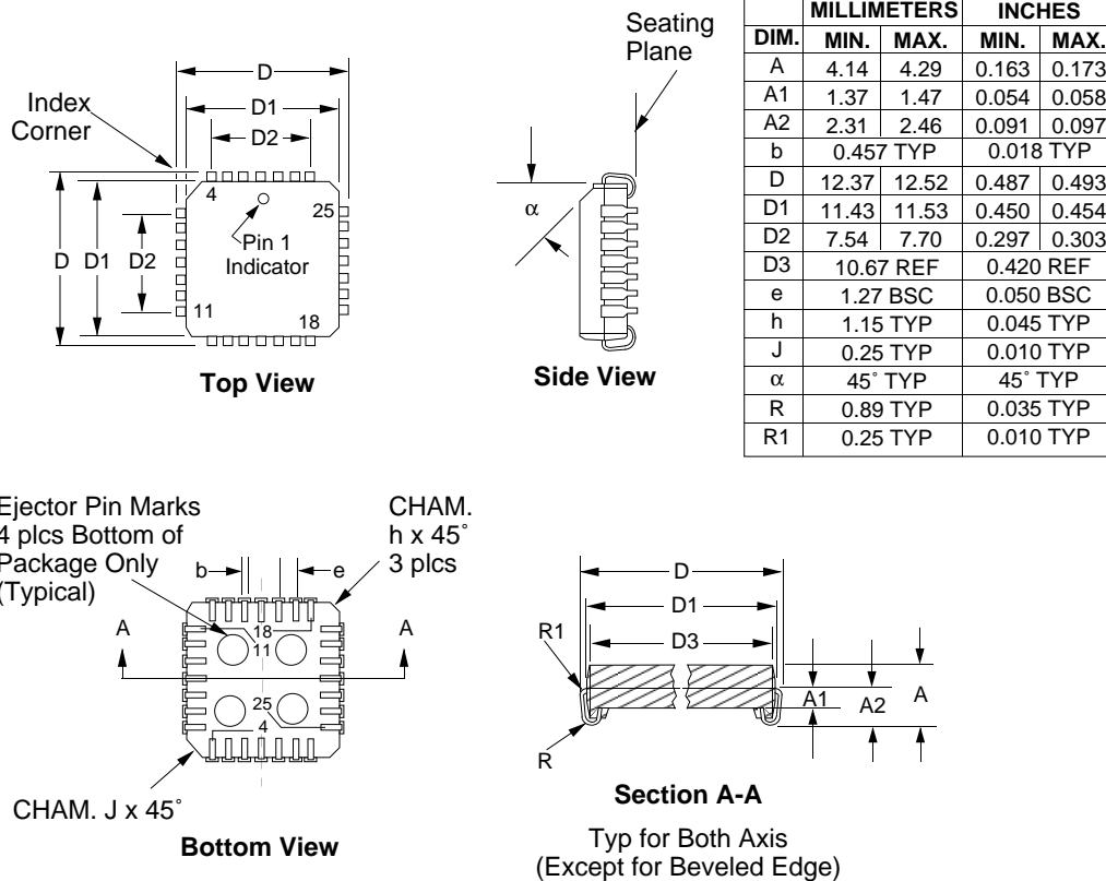
28-Pin PLCC
