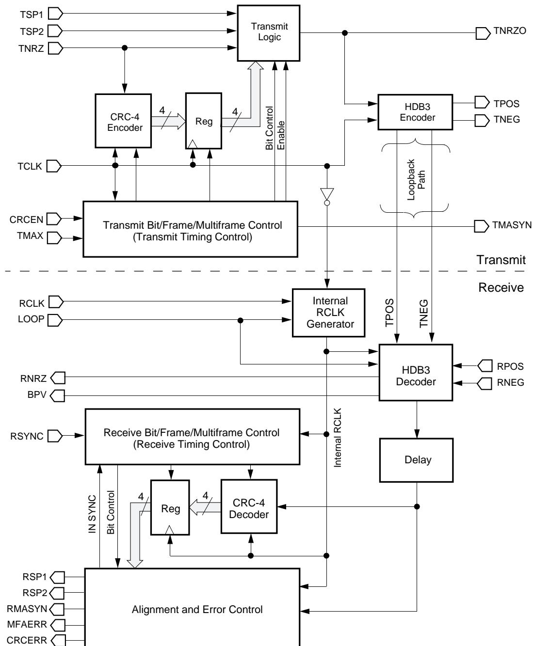
Figure 4. Bt8075 Functional Block Diagram
