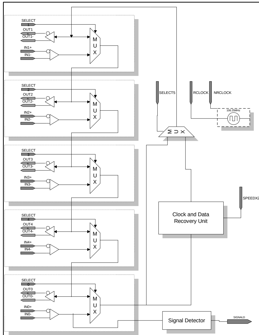
FIGURE 1 nLite BBT2010 Functional Block Diagram. SELECT5 determines whether the device is a Repeater or a Bypass Port.
