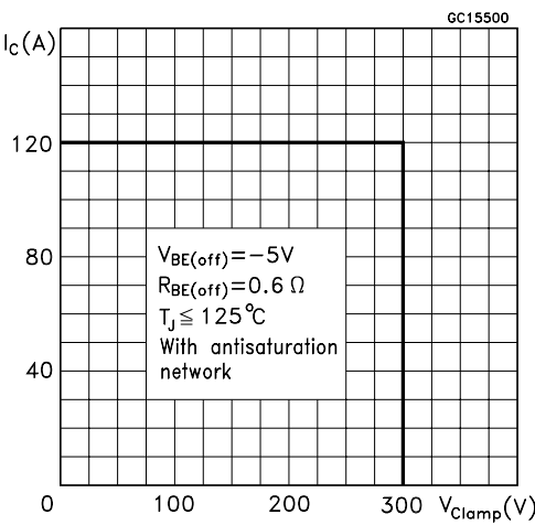
Reverse Biased AOA
