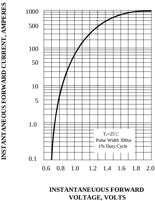
FIG 3 TYPICAL INSTANTANEOUS FORWRD CHARACTERISTICS
