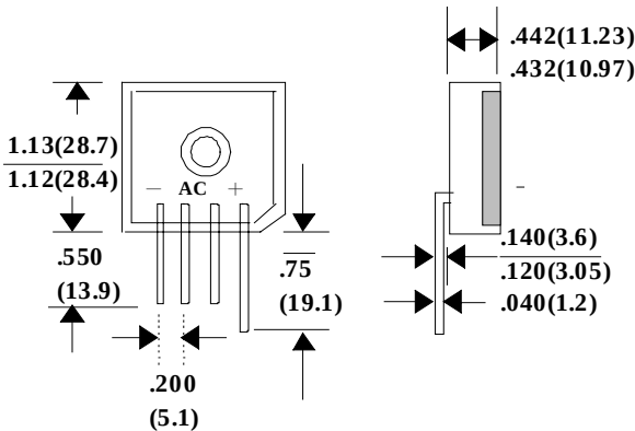
BL50-L IN LINE PIN CONFIGURATION (PLASTIC CASE)
