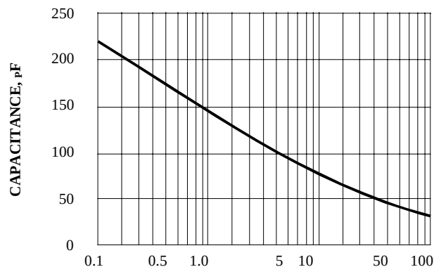
FIG. 5 - TYPICAL JUNCTION CAPACITANCE PER ELEMENT
