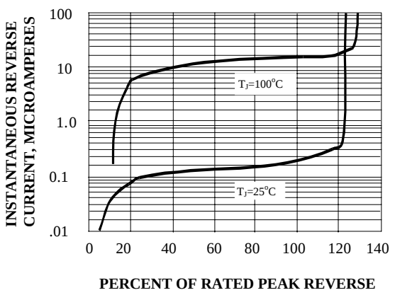
FIG. 3-TYPICAL REVERSE CHARACTERISTICS
