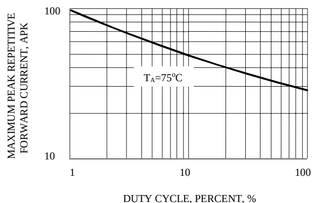
FIG. 3 - MAXIMUM PEAK REPETITIVE FORWARD SURGE CURRENT
