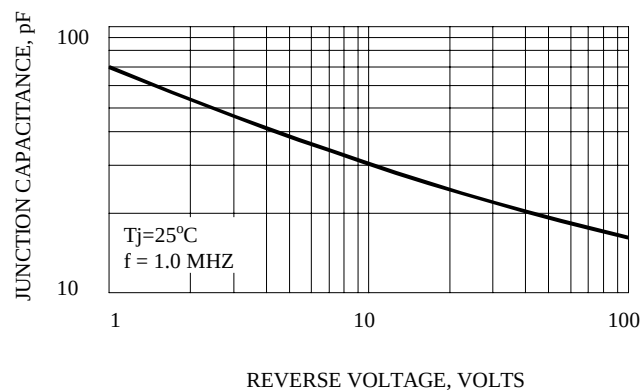
FIG. 6-TYPICAL JUNCTION CAPACITANCE
