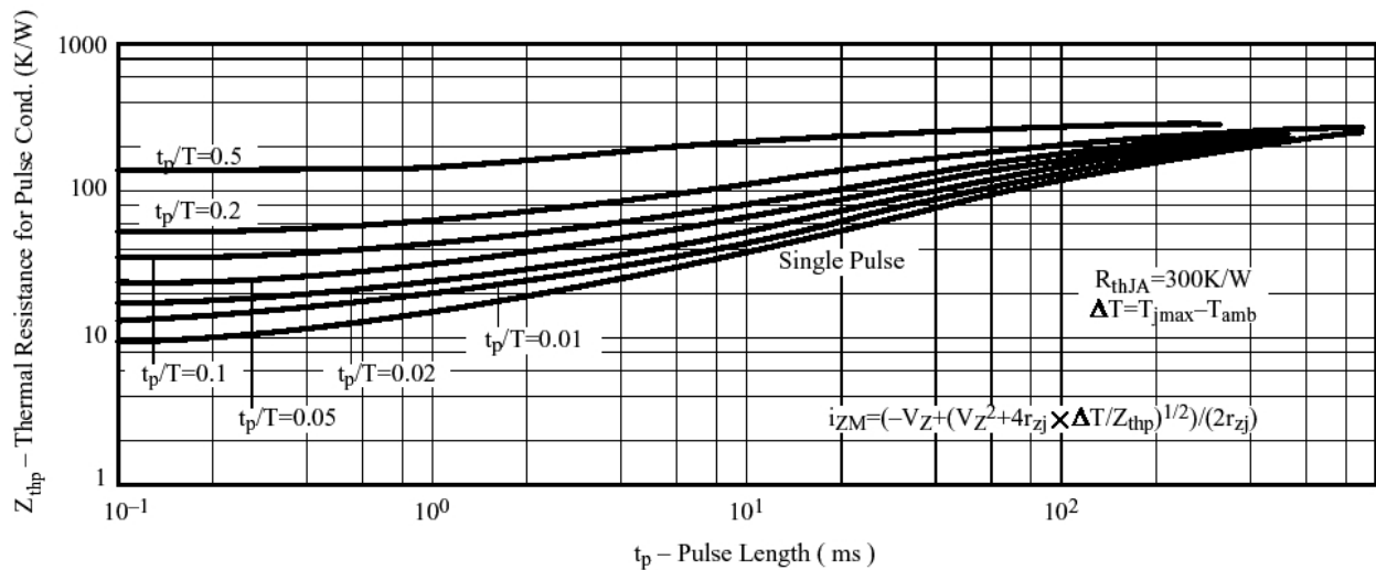
Figure 11. Thermal Response
