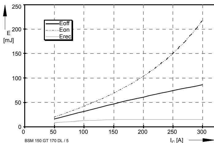
Bild / Fig. 5 Schaltverluste (typisch) / Switching losses (typical) E_{on} = f(I_C) , E_{off} = f(I_C) , E_{rec} = f(I_C) R_{gon} = R_{goff} = 10\Omega , V_{CE} = 900V , T_J = 125^\circ C
