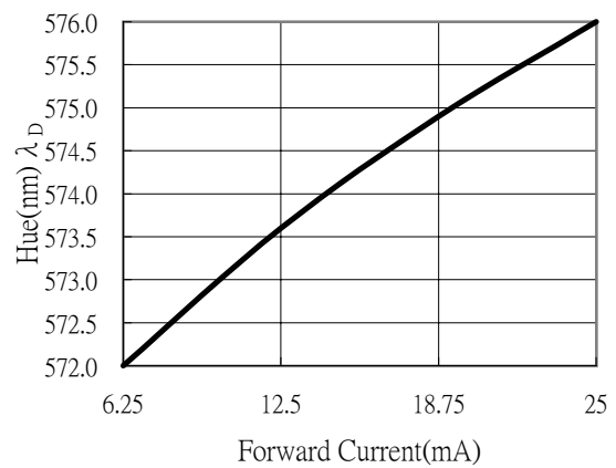
● Emission Wavelength vs. Forward Current ( T_a=25^{\circ}\text{C} )
