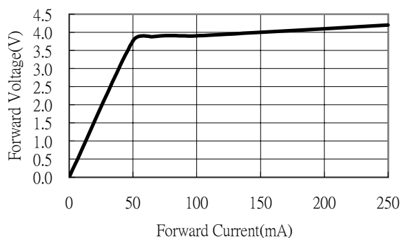
● Forward Voltage vs. Forward Current (Ta=25°C)
