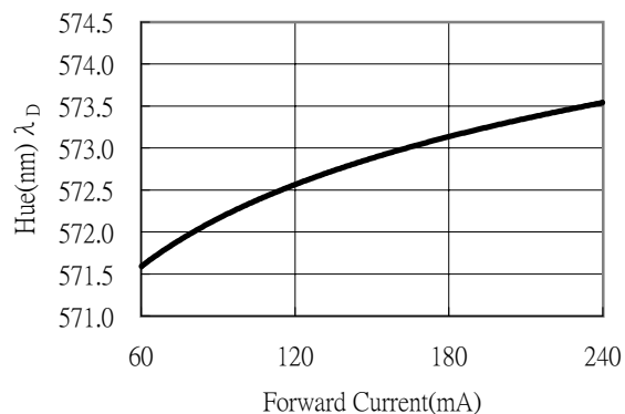
● Emission Wavelength vs. Forward Current (Ta=25°C)
