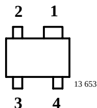
BFP67W Marking: W67 Plastic case (SOT 343) 1 = Collector, 2 = Emitter, 3 = Base, 4 = Emitter
