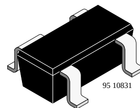
BFP67R Marking: 67R Plastic case (SOT 143R) 1 = Collector, 2 = Emitter, 3 = Base, 4 = Emitter
