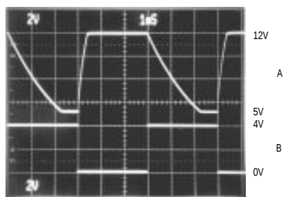
SHDN RESPONSE TIME
