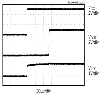
POWER-UP RESPONSE
