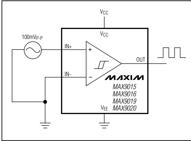
Figure 5. Zero-Crossing Detector
