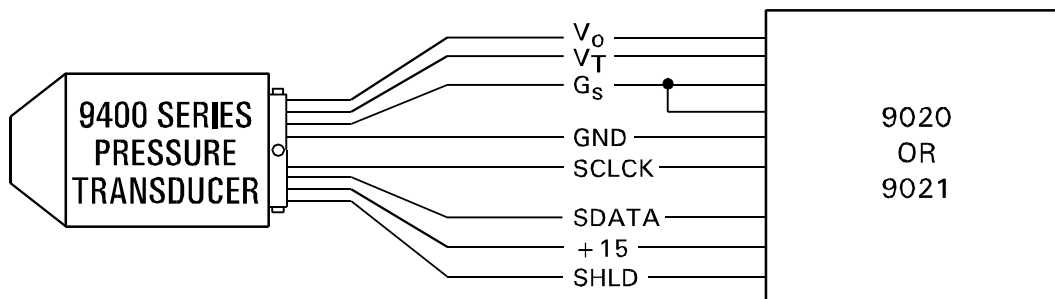
INTERFACE CONNECTION TO 9020 OR 9021
