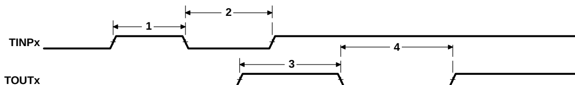
Figure 19–1. Timer Timing
