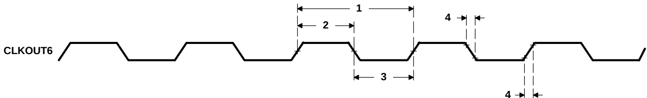
Figure 4–3. CLKOUT6 Timing
