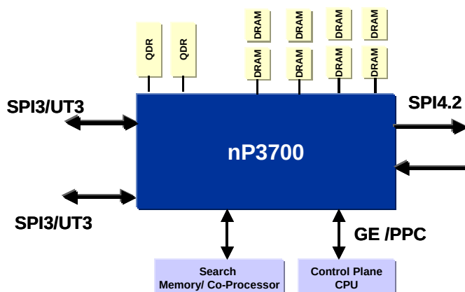
nP3700 Interface Diagram
