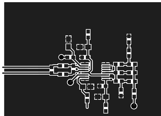
FIGURE 13. DEMO BOARD LAYOUT
