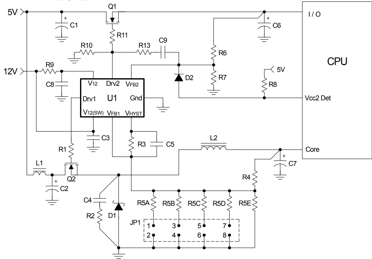
Figure 3 - Typical application of IRU3033 in a flexible motherboard with the 4-bit VID output voltage selection. This circuit uses a single jumper that programs the output voltage in 16 steps with 0.1V steps from 2V to 3.5V, designed for Intel P55™, P54™, AMD K5 & K6™ as well as Cyrix M1™ and M2™ applications. The Vcc2 Det pin automatically shuts down the I/O regulator when a single plane processor is dropped in the socket.
