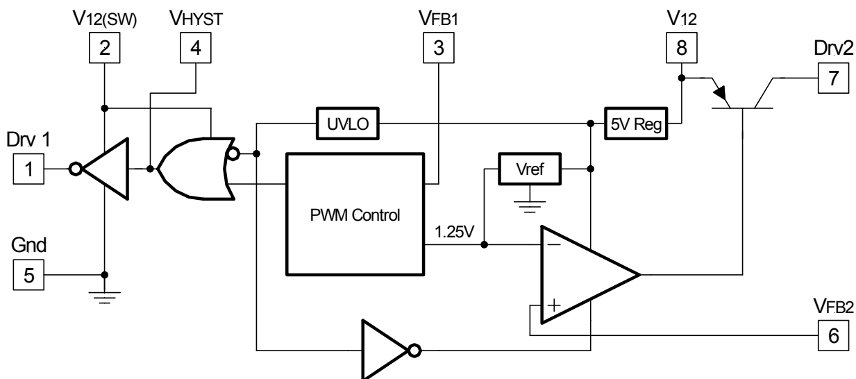
Figure 2 - Simplified block diagram of the IRU3033.
