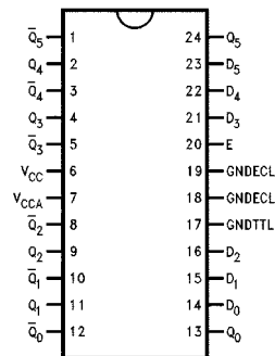
24-Pin DIP and SOIC
