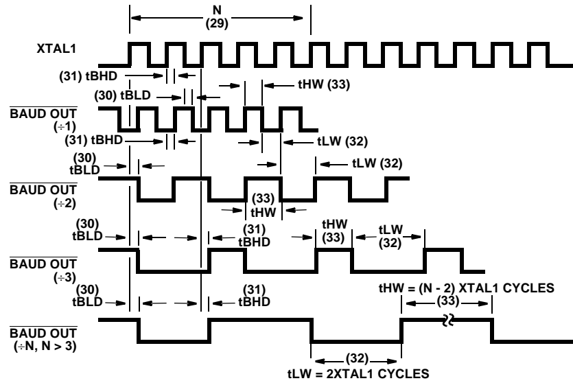
FIGURE 5. BAUDOUT TIMING
