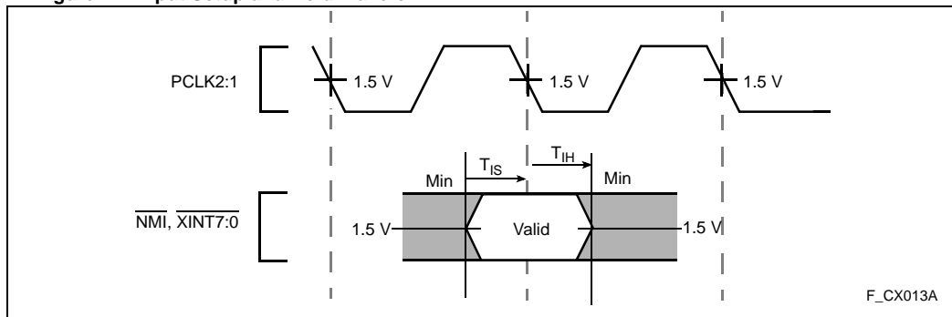
Figure 12. \overline{\text{NMI}} , \overline{\text{XINT7:0}} Input Setup and Hold Waveform
