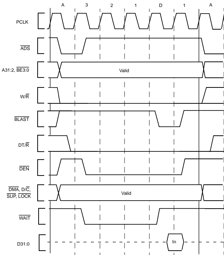
Figure 26. Non-Burst, Non-Pipelined Read Request With Wait States
