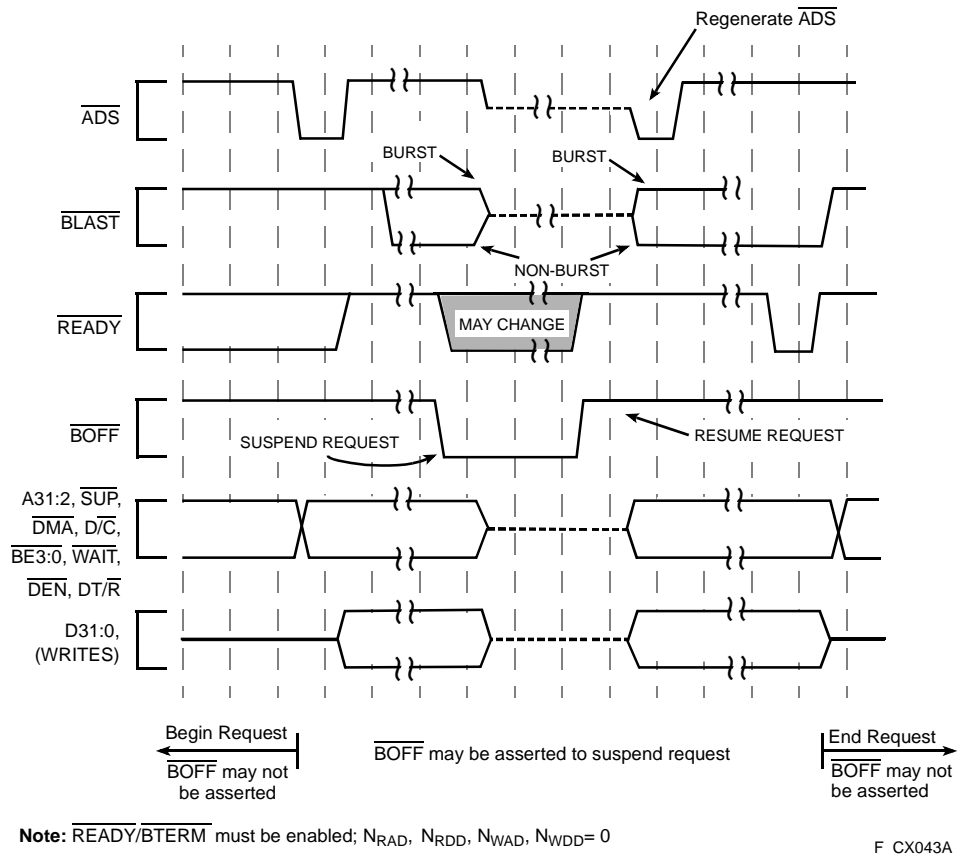
Figure 42. \overline{\text{BOFF}} Functional Timing
