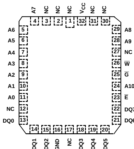
HM-65162 (CLCC) TOP VIEW
