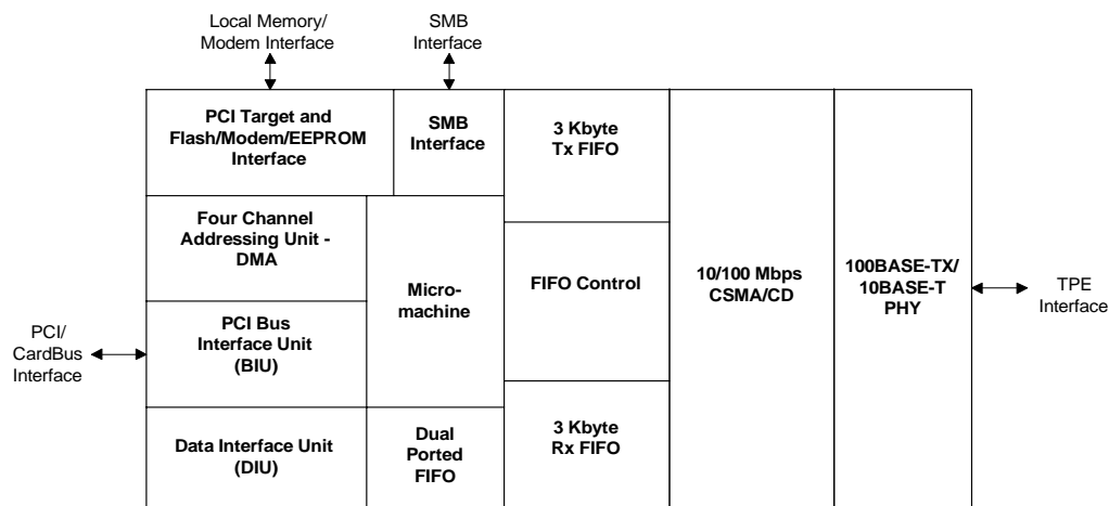
Figure 1. 82559 Block Diagram
