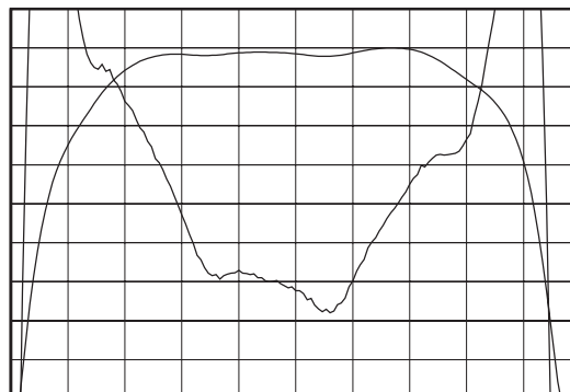
Horizontal: 75 kHz/Div Vertical: 1 dB/Div Vertical: 100 nsec/Div
