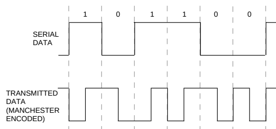
Figure 2. Manchester Coding
