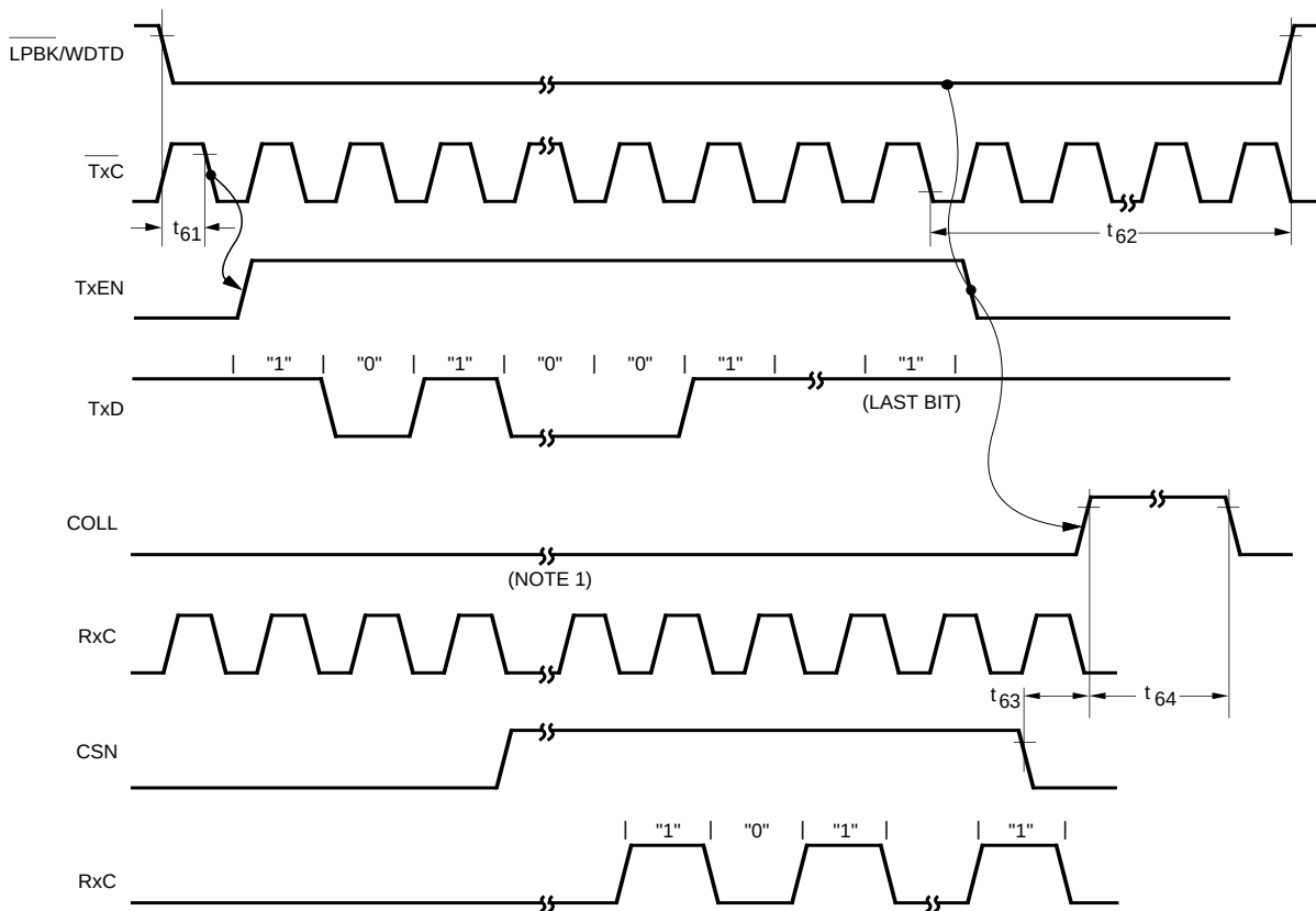
Figure 12. Loopback Timing
