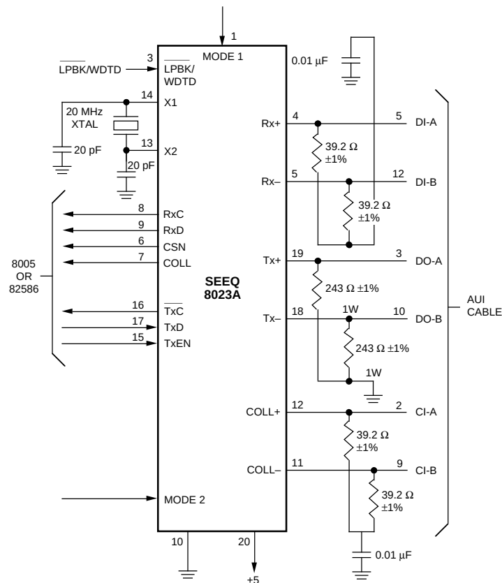
Figure 4. 8023A Interface
