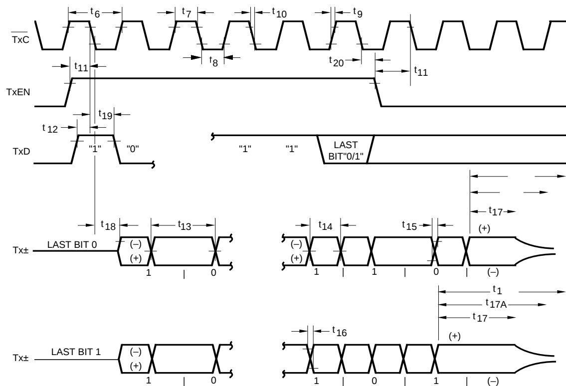
Figure 7. Transmit Timing
