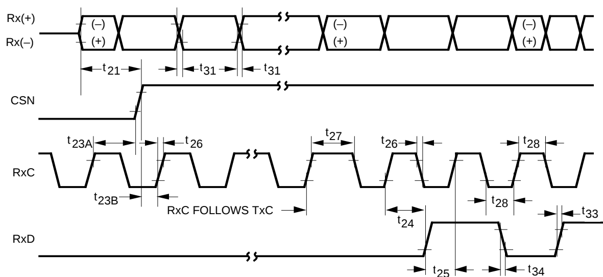
Figure 9. Receive Timing-Start of Packet
