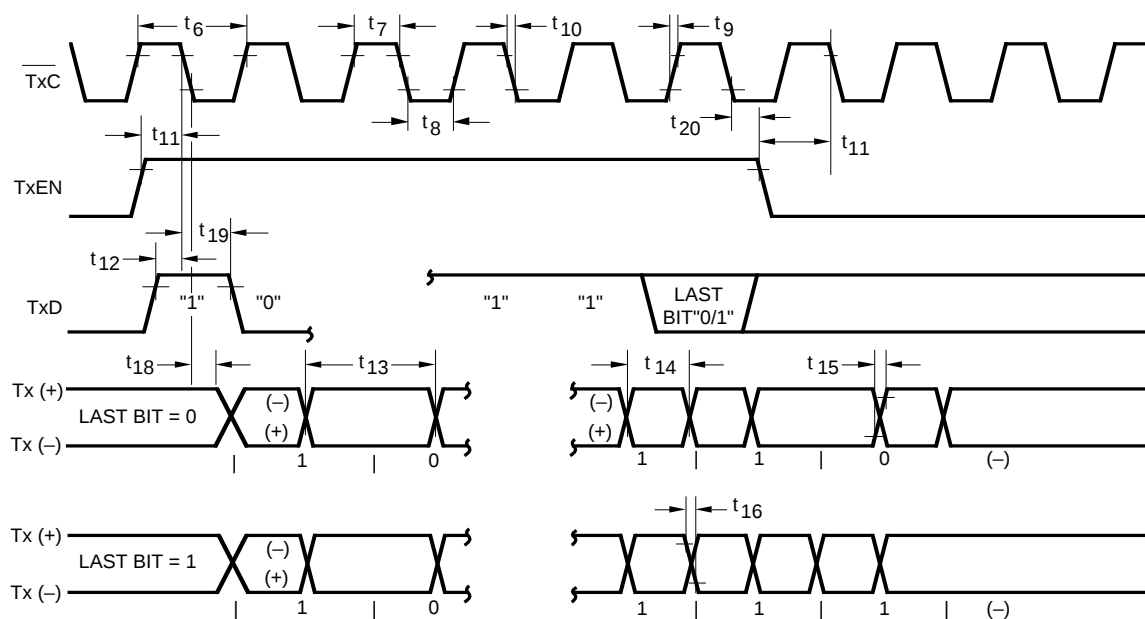
Figure 8. Transmit Timing
