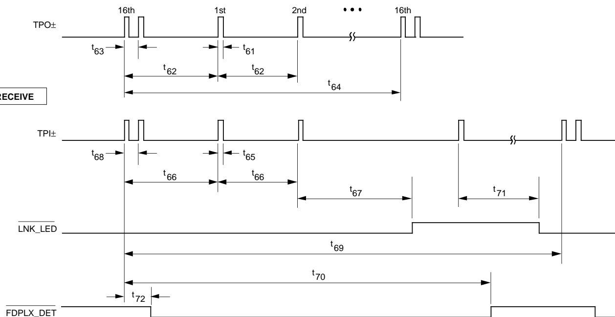
Figure 9. Link Pulse Timing
