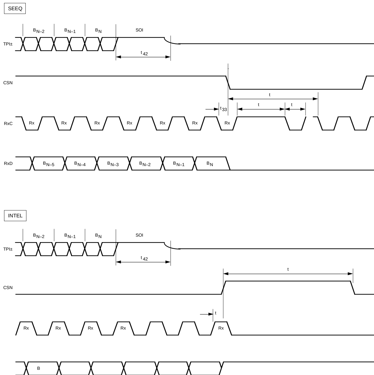
Figure 13. Receive Timing, End of Packet
