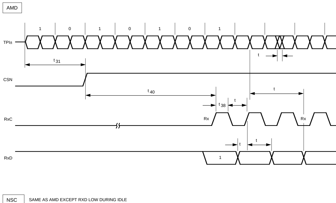
Figure 12. Receive Timing, Start of Packet (continued)
