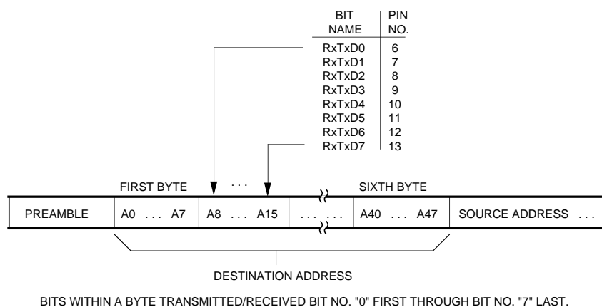
Figure 4. Bit Serialization/Deserialization
