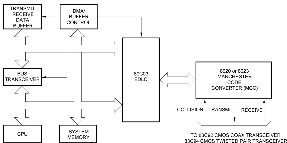
Figure 5. Typical Ethernet Node Configuration
