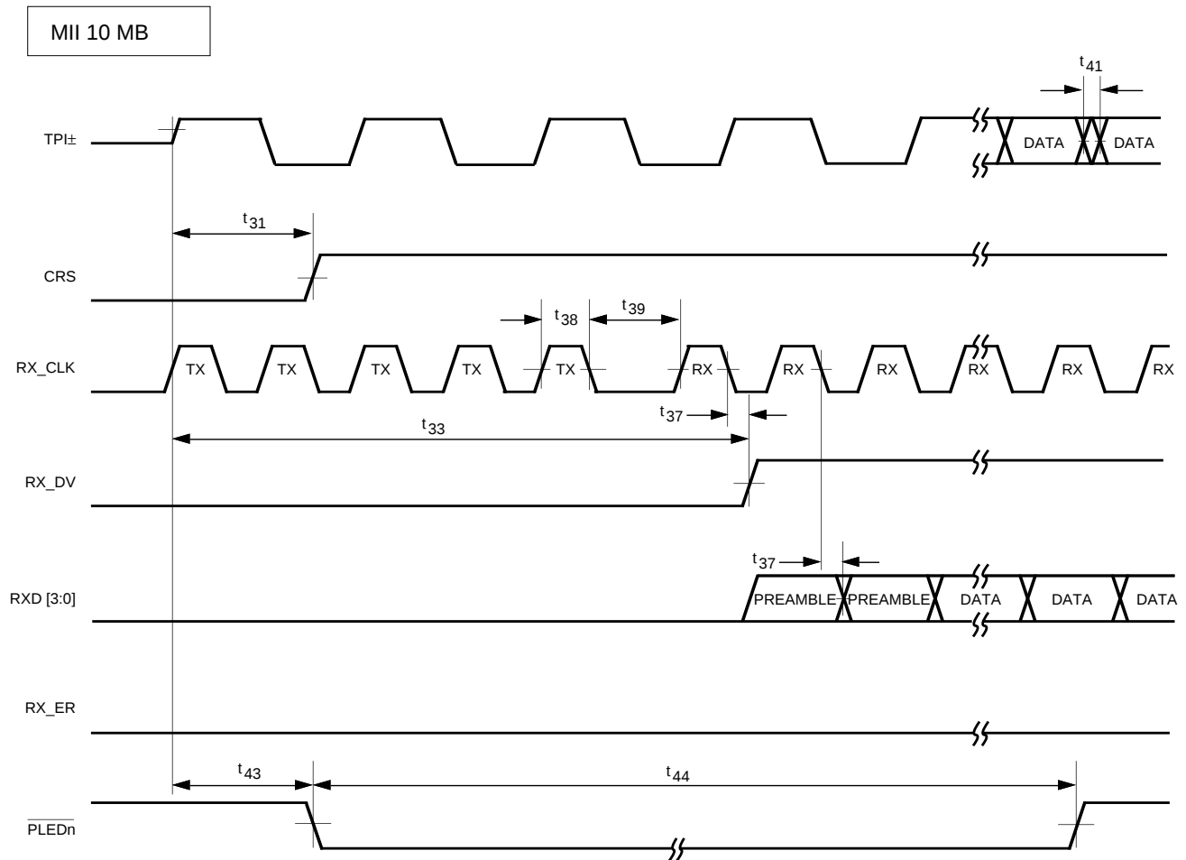
Figure 21. Receive Timing, Start of Packet - 10 Mbps
