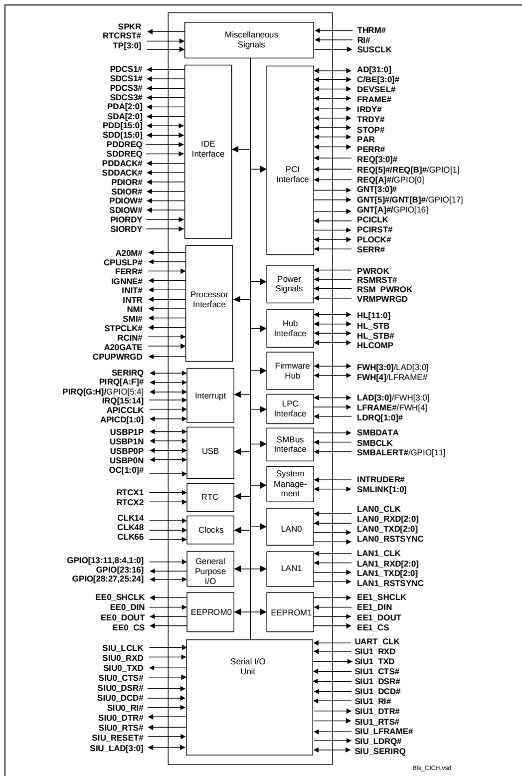
Figure 2. 82801E C-ICH Simplified Block Diagram
