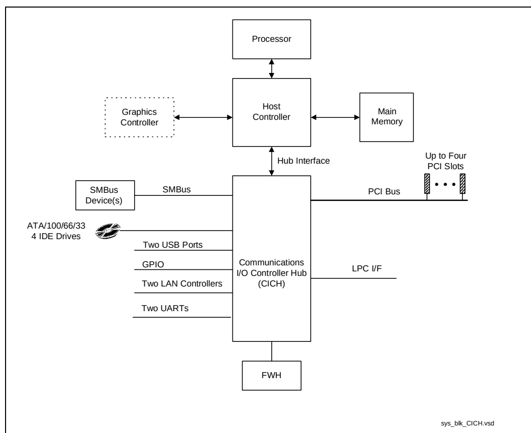
Figure 1. System Configuration
