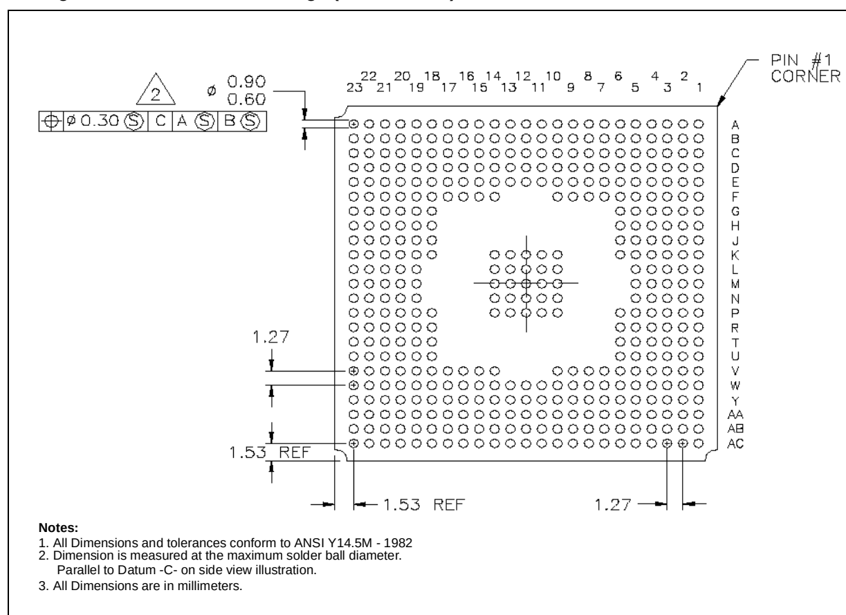
Figure 6. 82801E C-ICH Package (Bottom View)
