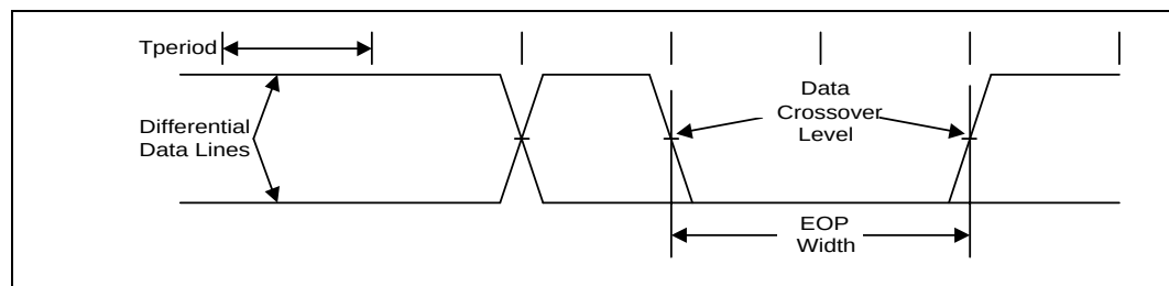
Figure 24. SMBus Transaction
