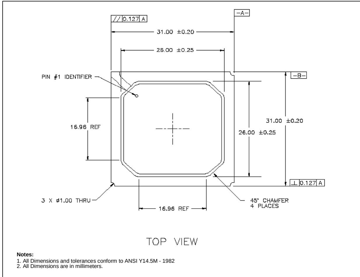
Figure 4. 82801E C-ICH Package (Top View)
