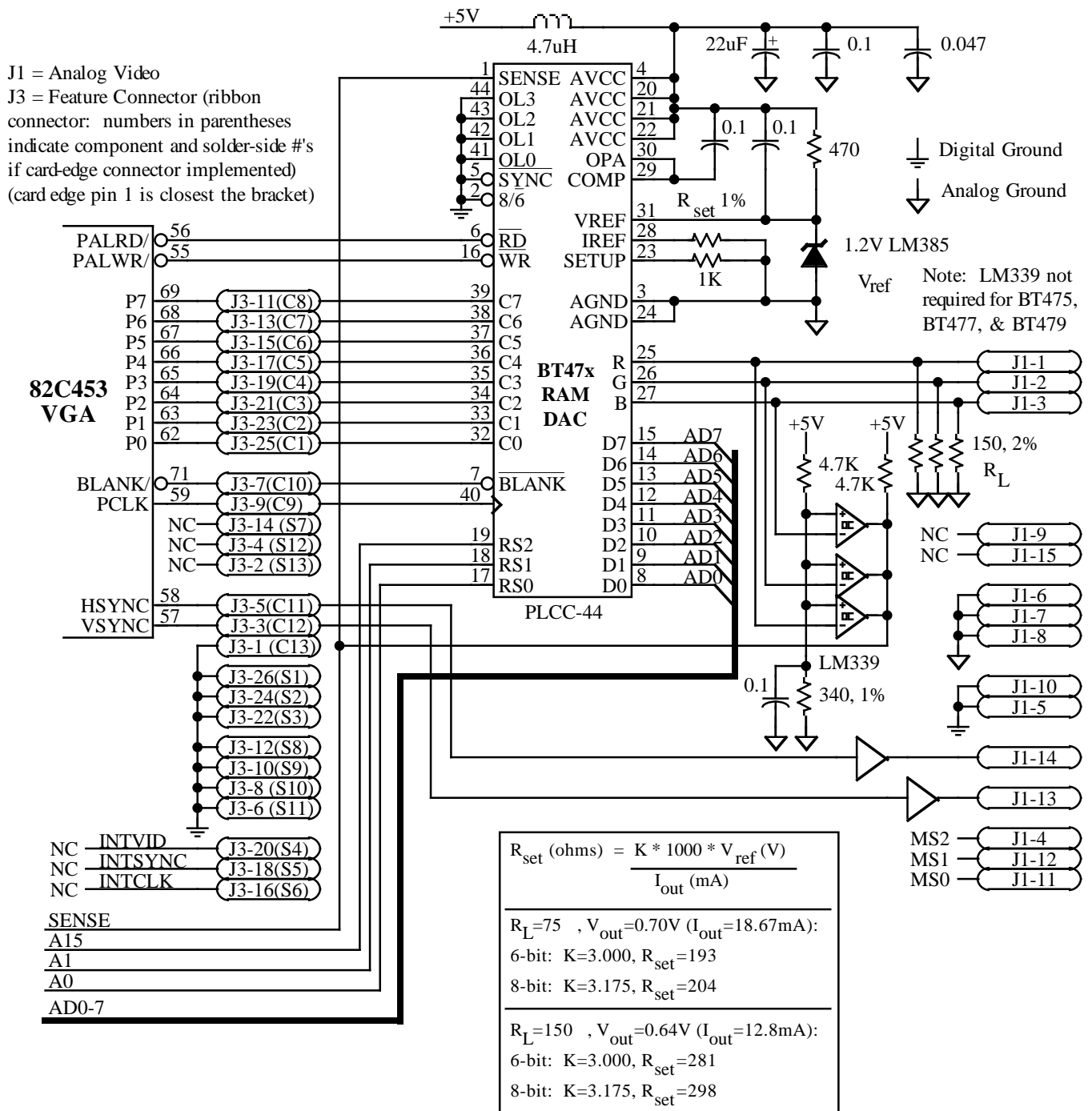
82C453 Video Circuit Example - External Color Palette (Brooktree BT471 / 475 / 477 / 478 / 479)
