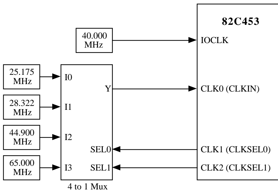
Block Diagram - External Clock Multiplexer Interface
