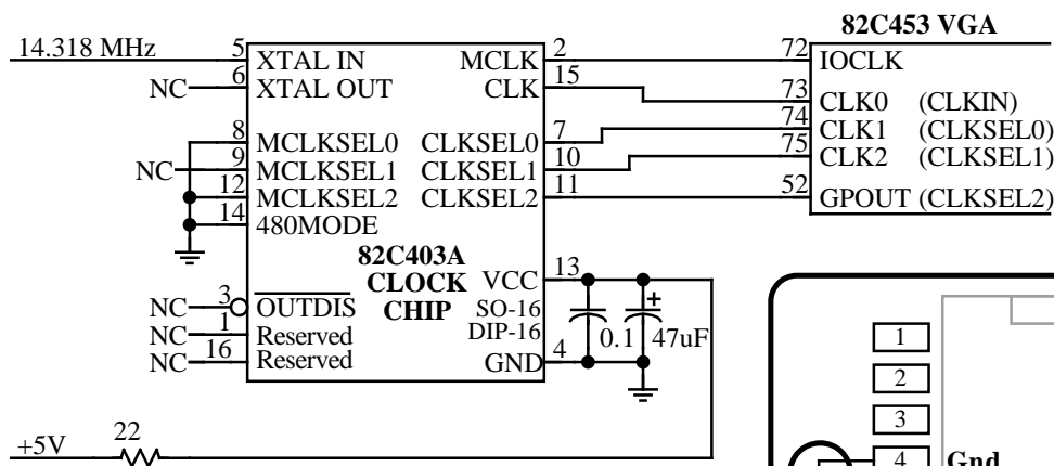
82C453 Clock Circuit Example - Full Oscillator Configuration
