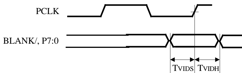
82C453 Video Data Timing
