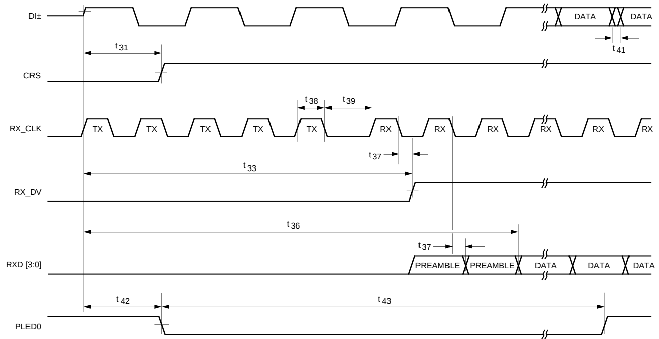
Figure 15. Receive Timing, Start of Packet
