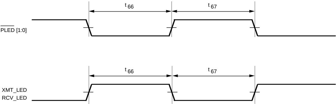
Figure 19. LED Driver Timing
