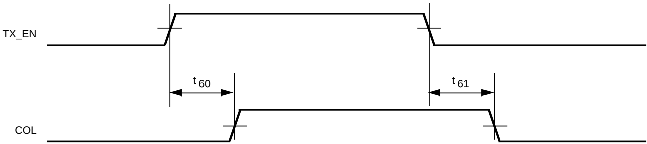
Figure 18. Collision Test Timing
