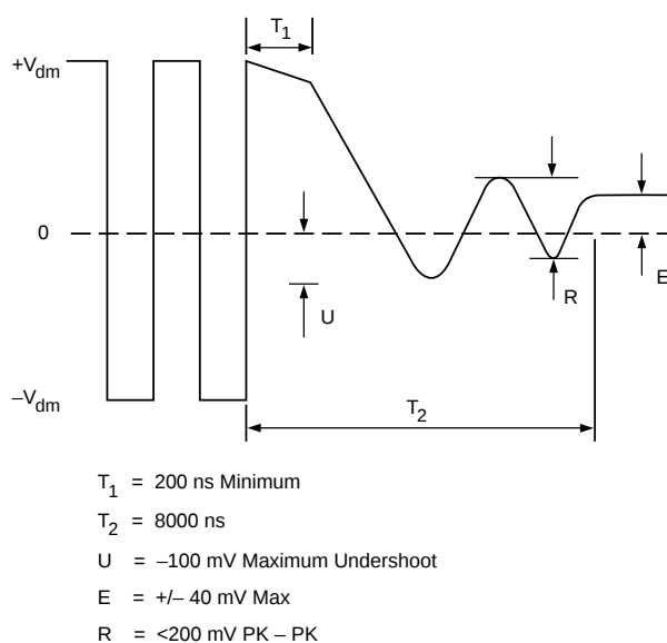
Figure 4. AUI Transmit SOI Output Voltage Template
