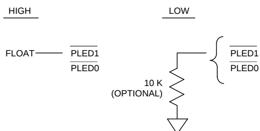
Figure 12. MI Serial Port Address Selection
