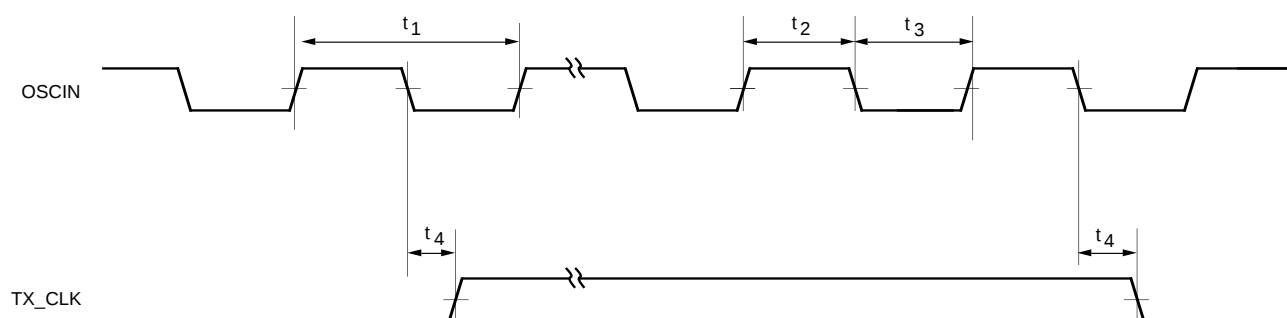
Figure 13. 20 MHz Clock Timing
