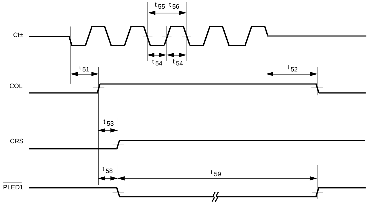
Figure 17. Collision Timing
