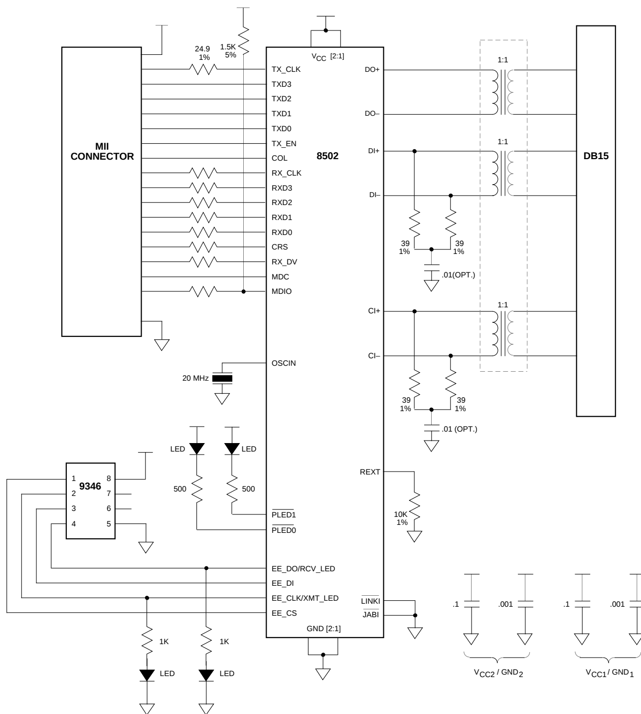
Figure 8. External MII-AUI Schematic Using 8502 with EEPROM and LED's
