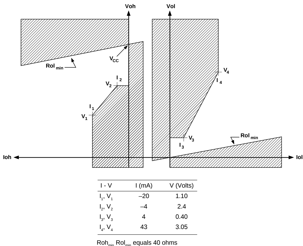
Figure 11. MII Output Driver Characteristics
