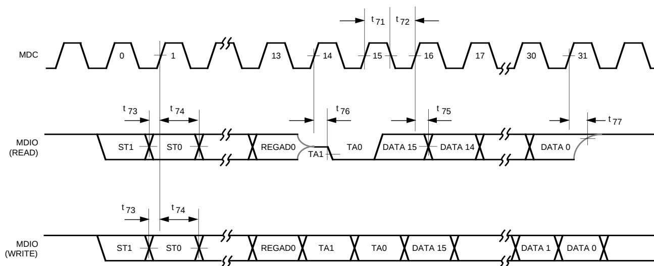
Figure 20. MI Serial Port Timing
