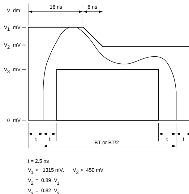
Figure 3. AUI Transmit Output Voltage Template
