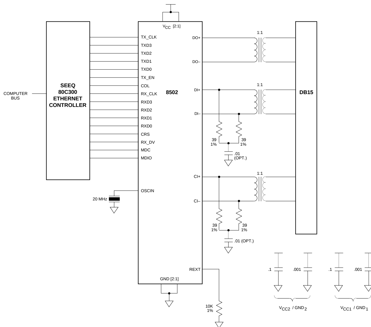
Figure 10. Network Interface Card Schematic Using 8502
