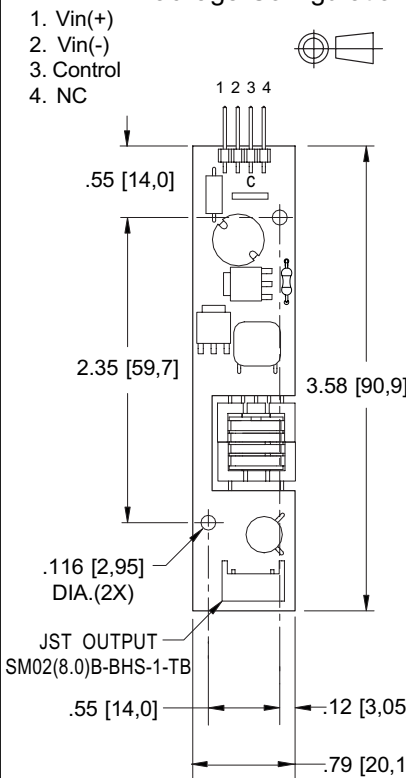
8m Package
