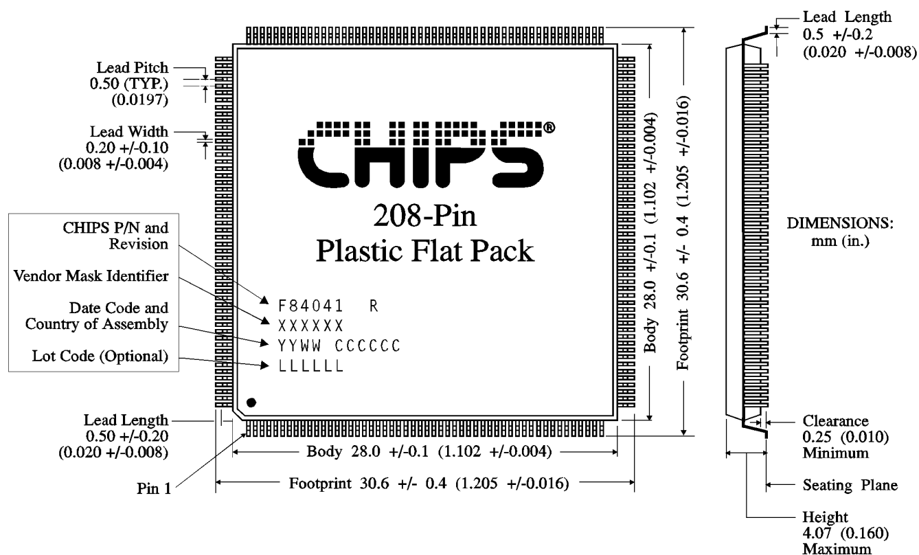
Figure 8.6: 84041 Packaging Dimensions
