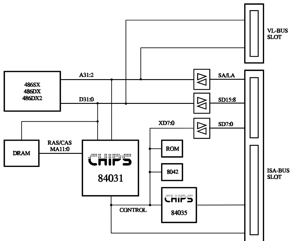
System Diagram
