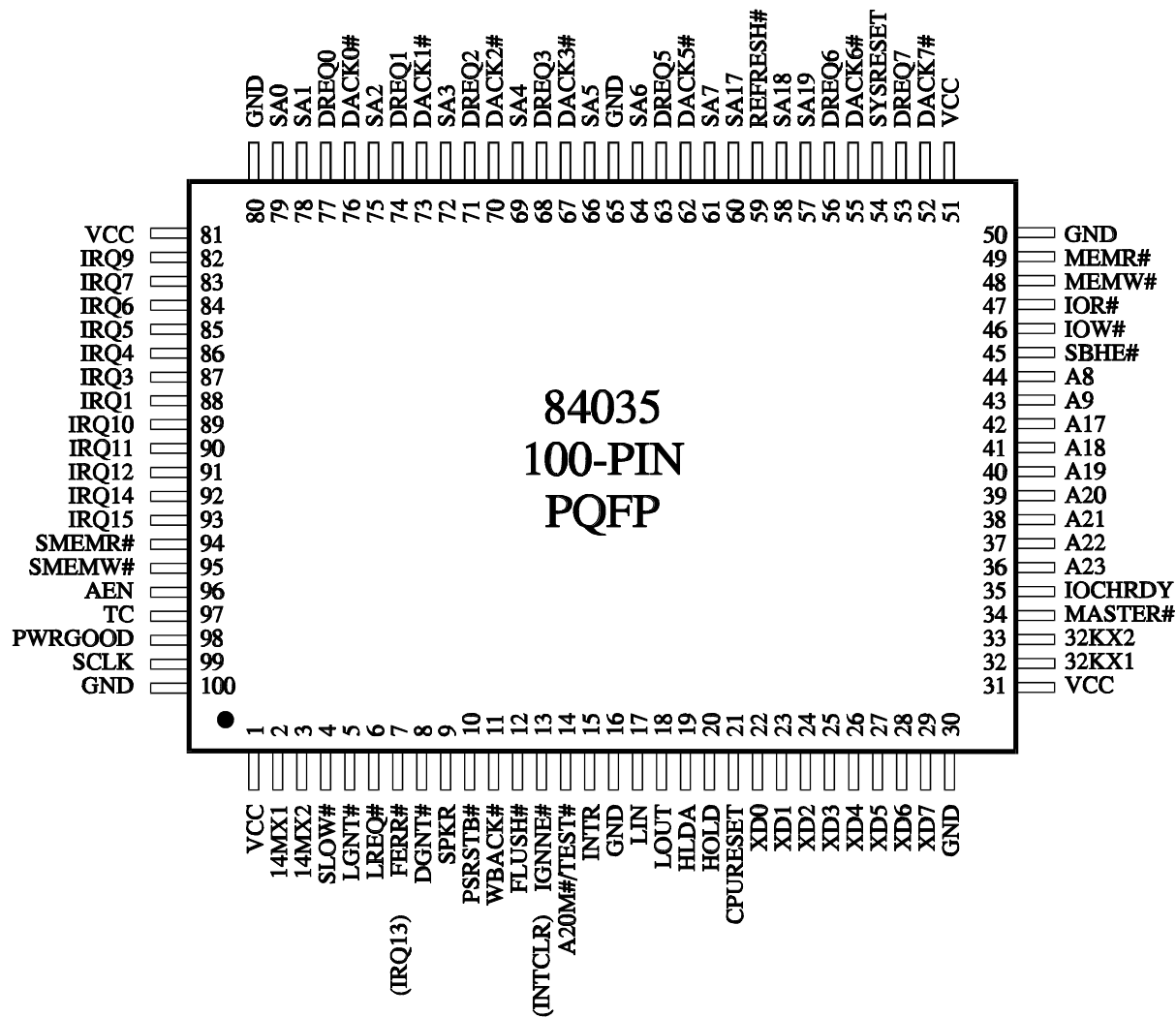
84035 Pinout
