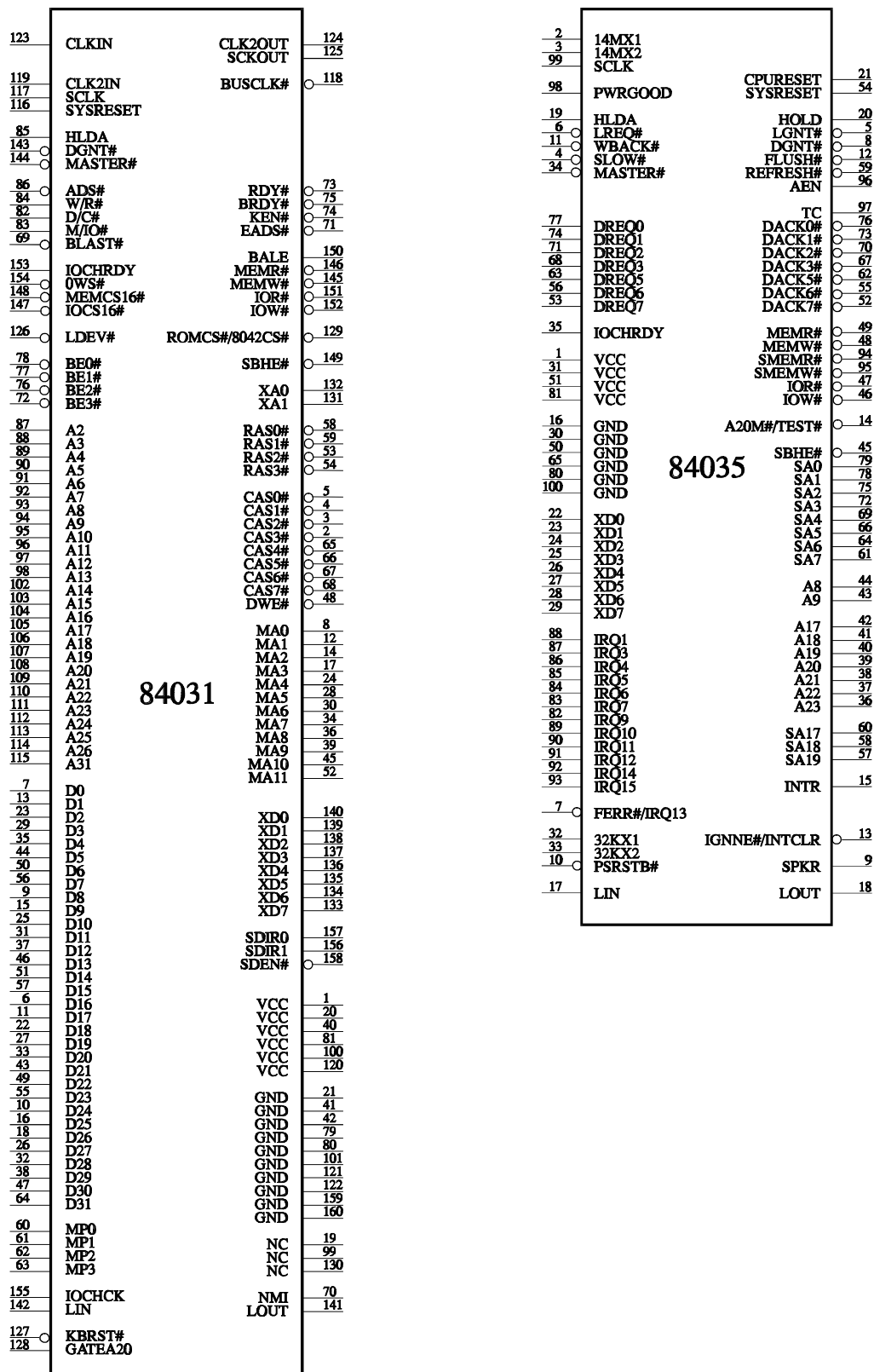
Schematic Symbols
