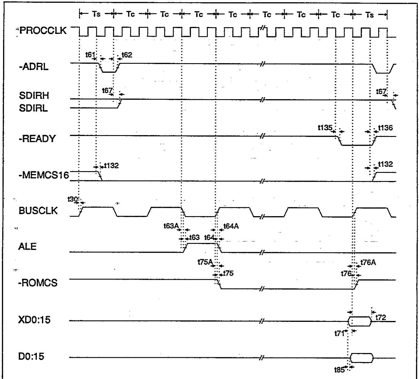
Figure 10-7. 16-Bit ROM Cycle
