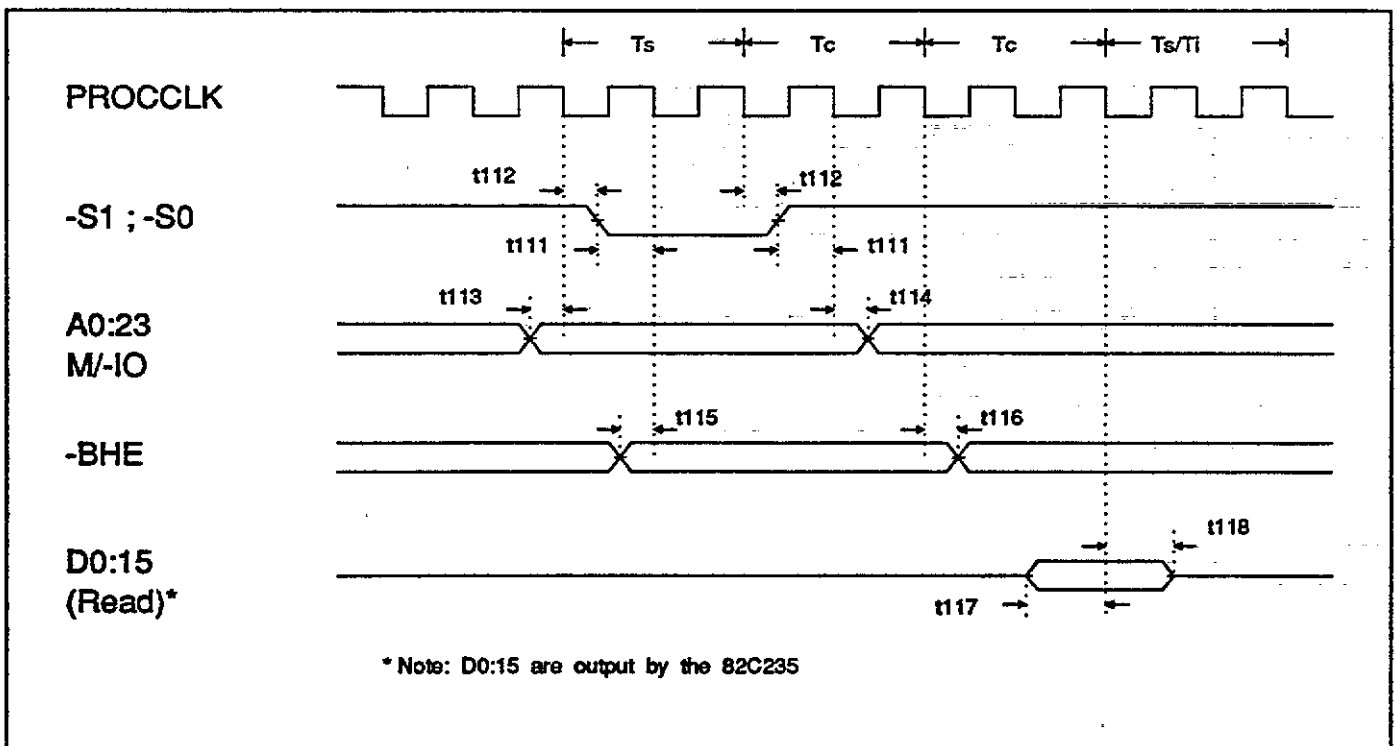
Figure 10-11. CPU Interface
