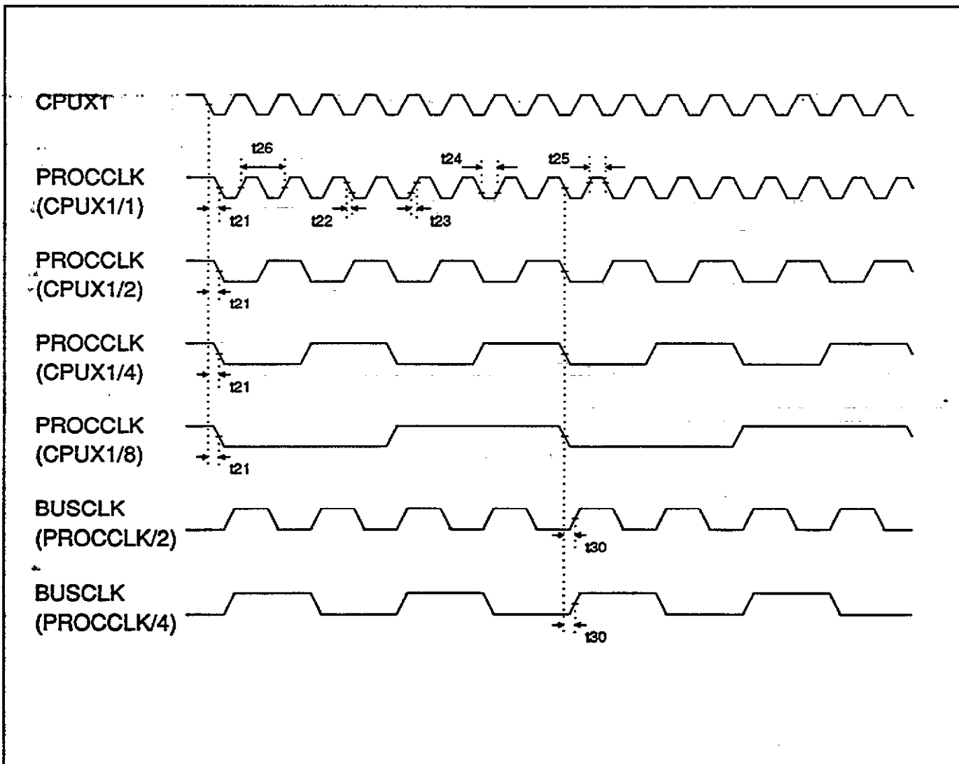
Figure 10-3. Clock Output
