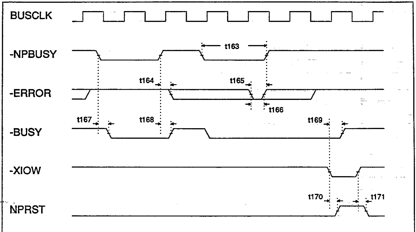
Figure 10-11. CPU Interface
