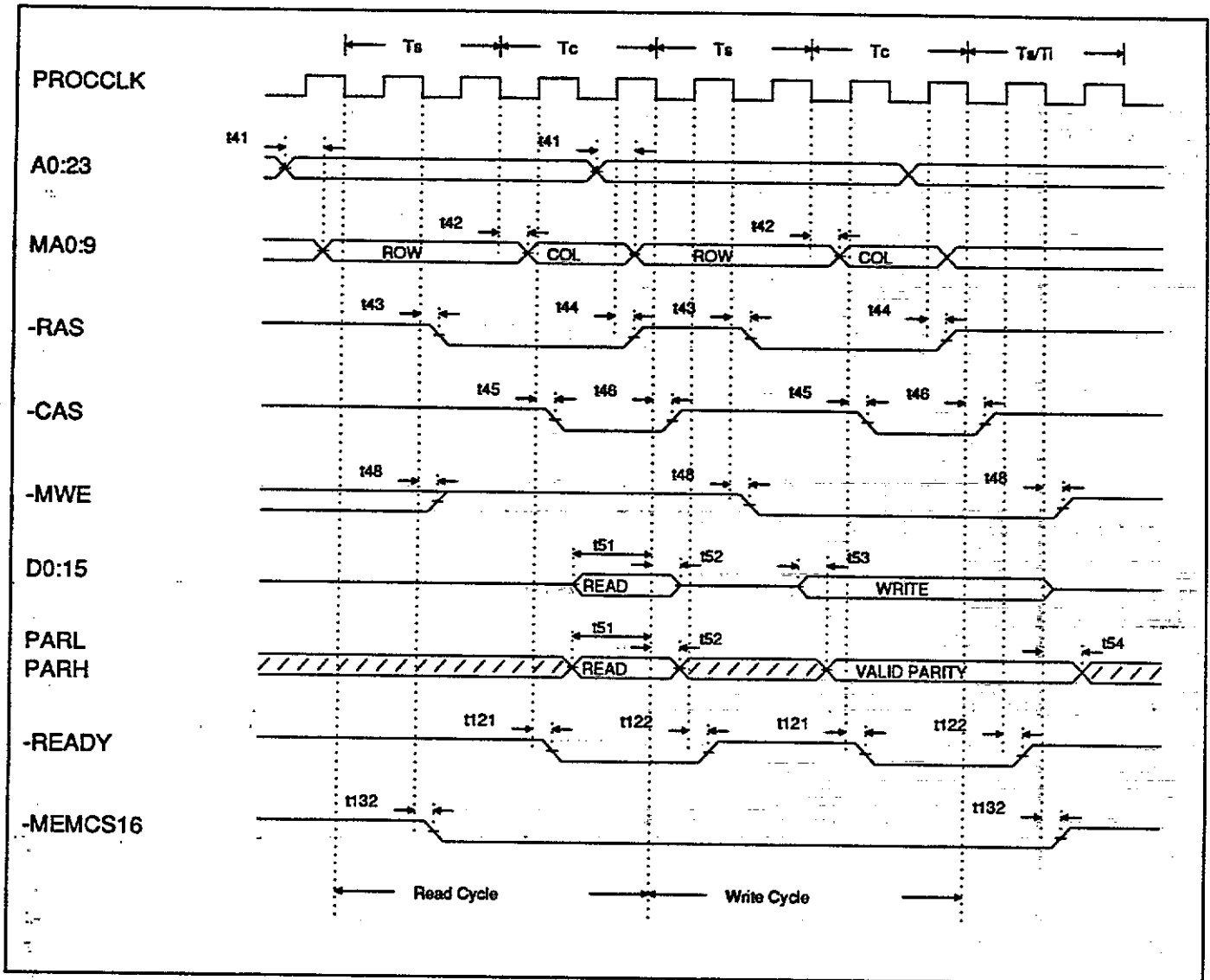
Figure B-2. Zero Wait State DRAM - Revision A Silicon
