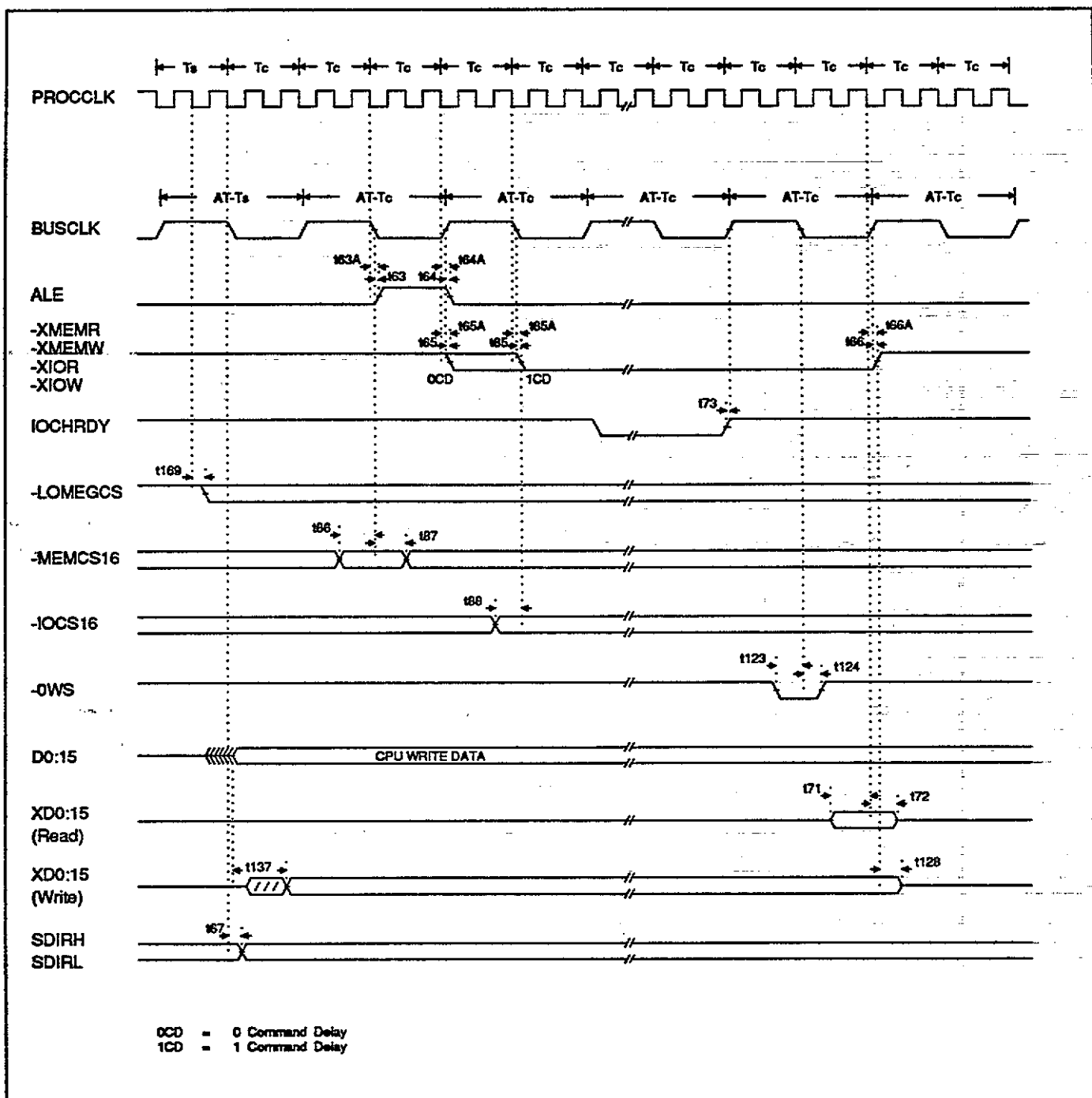
Figure 10-14. I/O Channel
