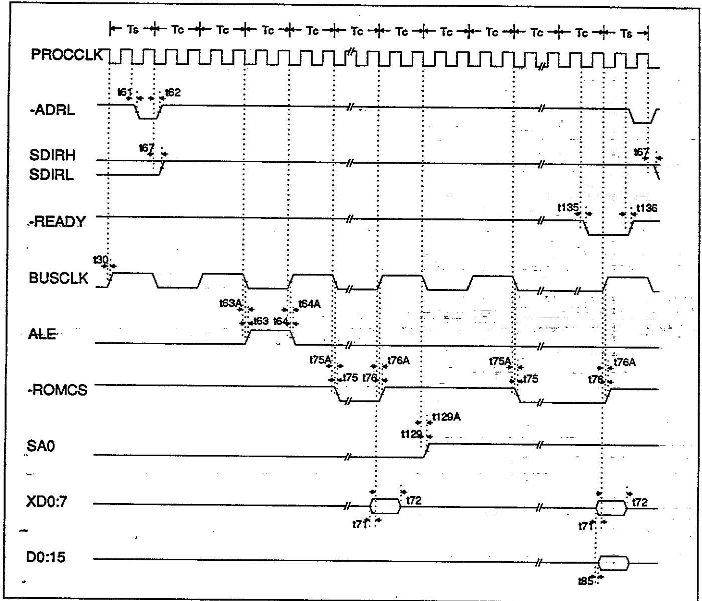
Figure 10-8. 8-Bit ROM Cycle
