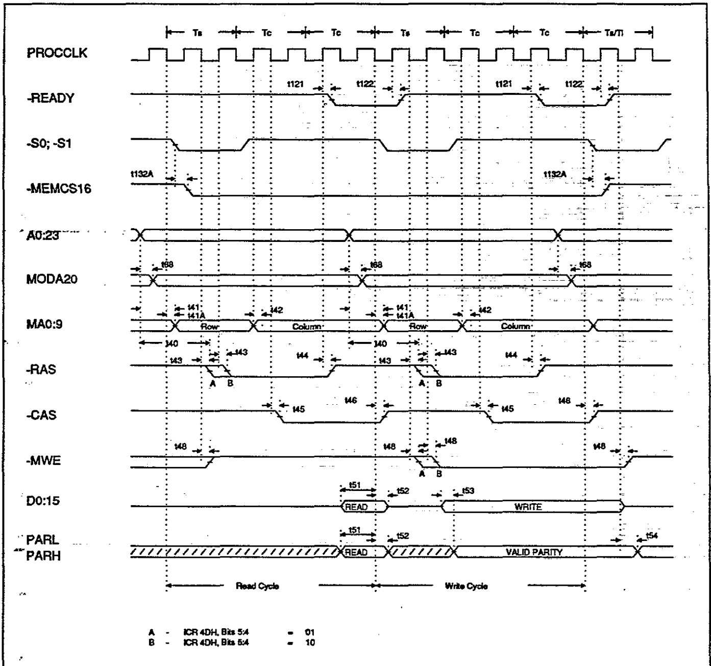
Figure 10-6. One Wait State DRAM
