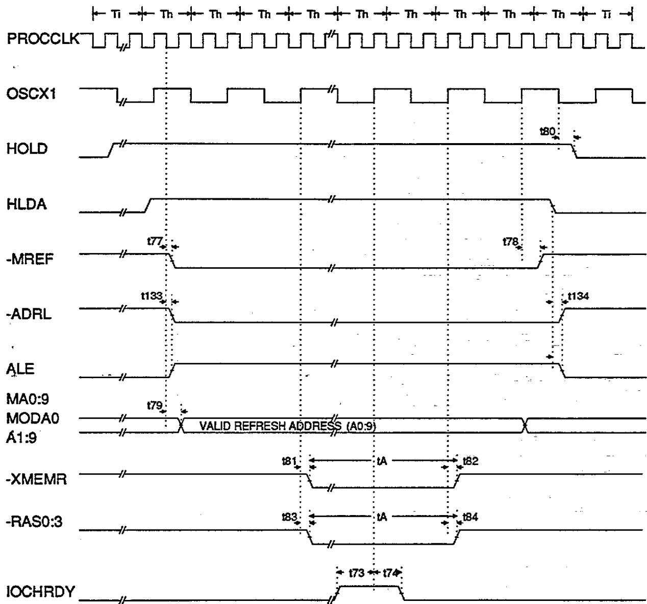
Figure 10-9. Memory Refresh Cycle
