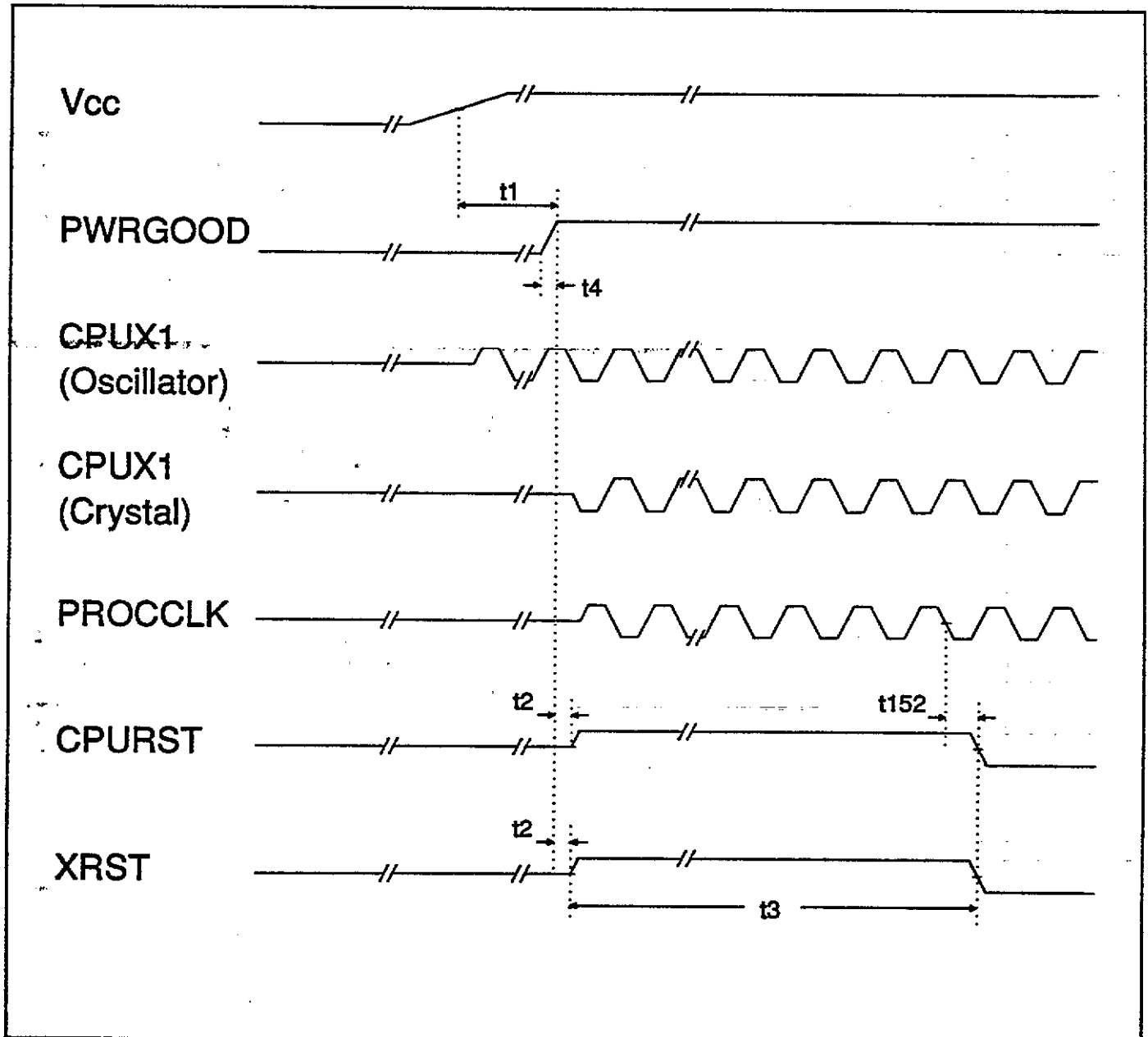
Figure 10-1. Hardware Reset
