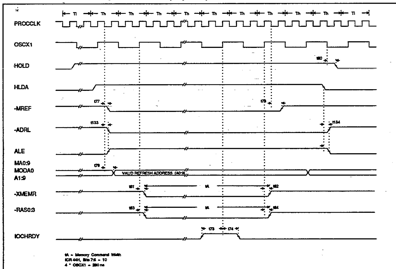
Figure B-1. Memory Refresh Cycle - Revision A Silicon
