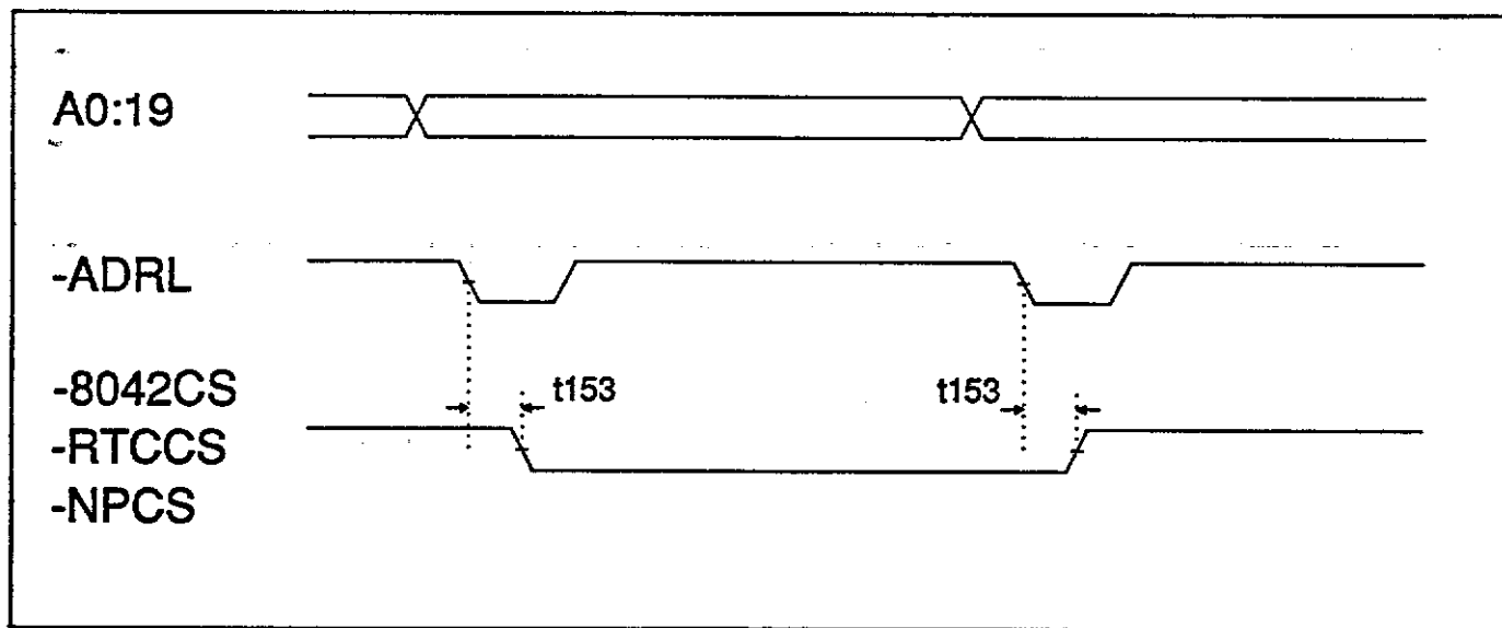
Figure 10-13. Peripheral Control
