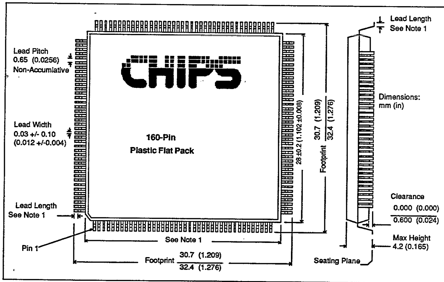
Figure 11-1. 160-Pin Plastic Flat Package
