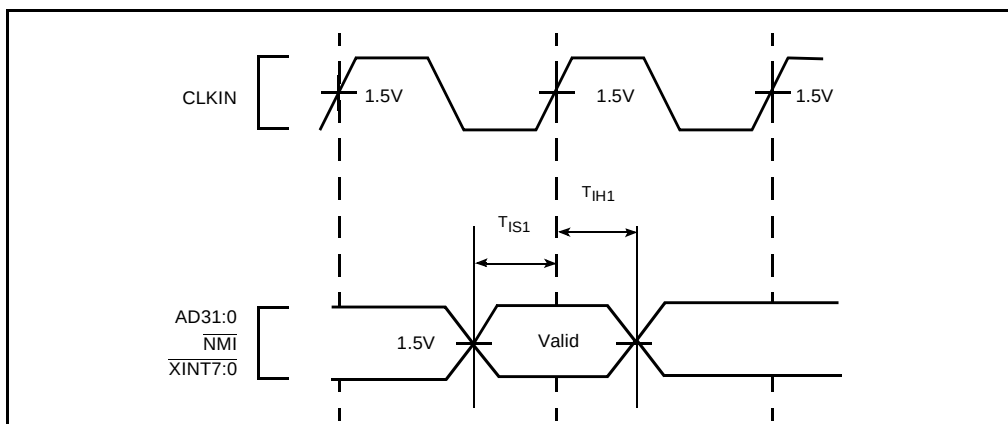
Figure 13. Input Setup and Hold Waveform for T_{IS1} and T_{IH1}
