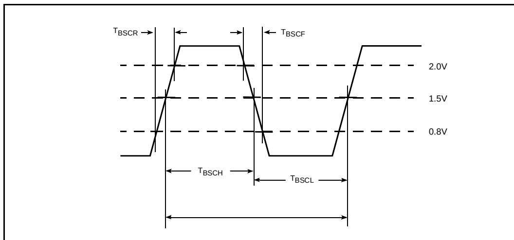
Figure 19. TCK Waveform
