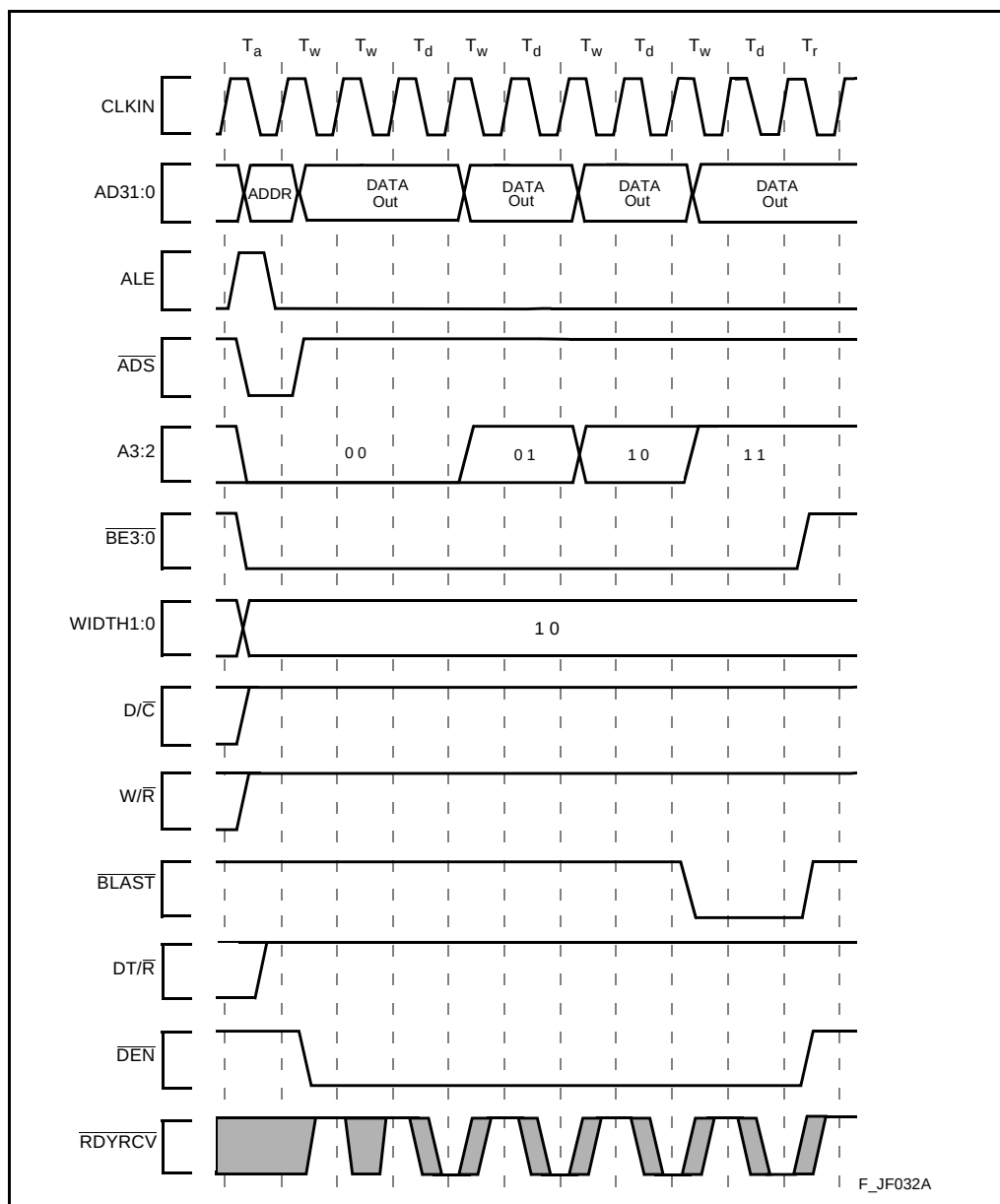
Figure 26. Burst Write Transactions With 2,1,1,1 Wait States, 32-Bit Bus
