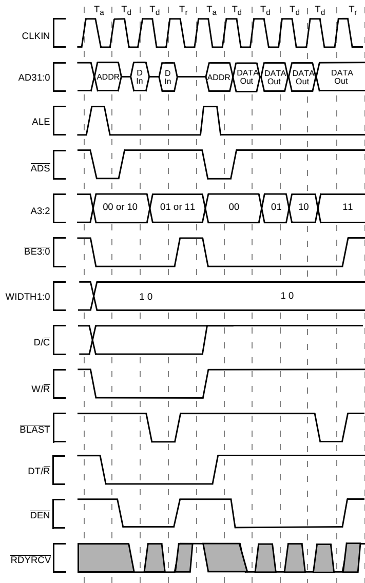
Figure 25. Burst Read and Write Transactions Without Wait States, 32-Bit Bus
