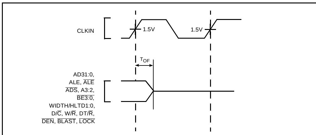
Figure 12. Output Float Waveform for T_{OF}
