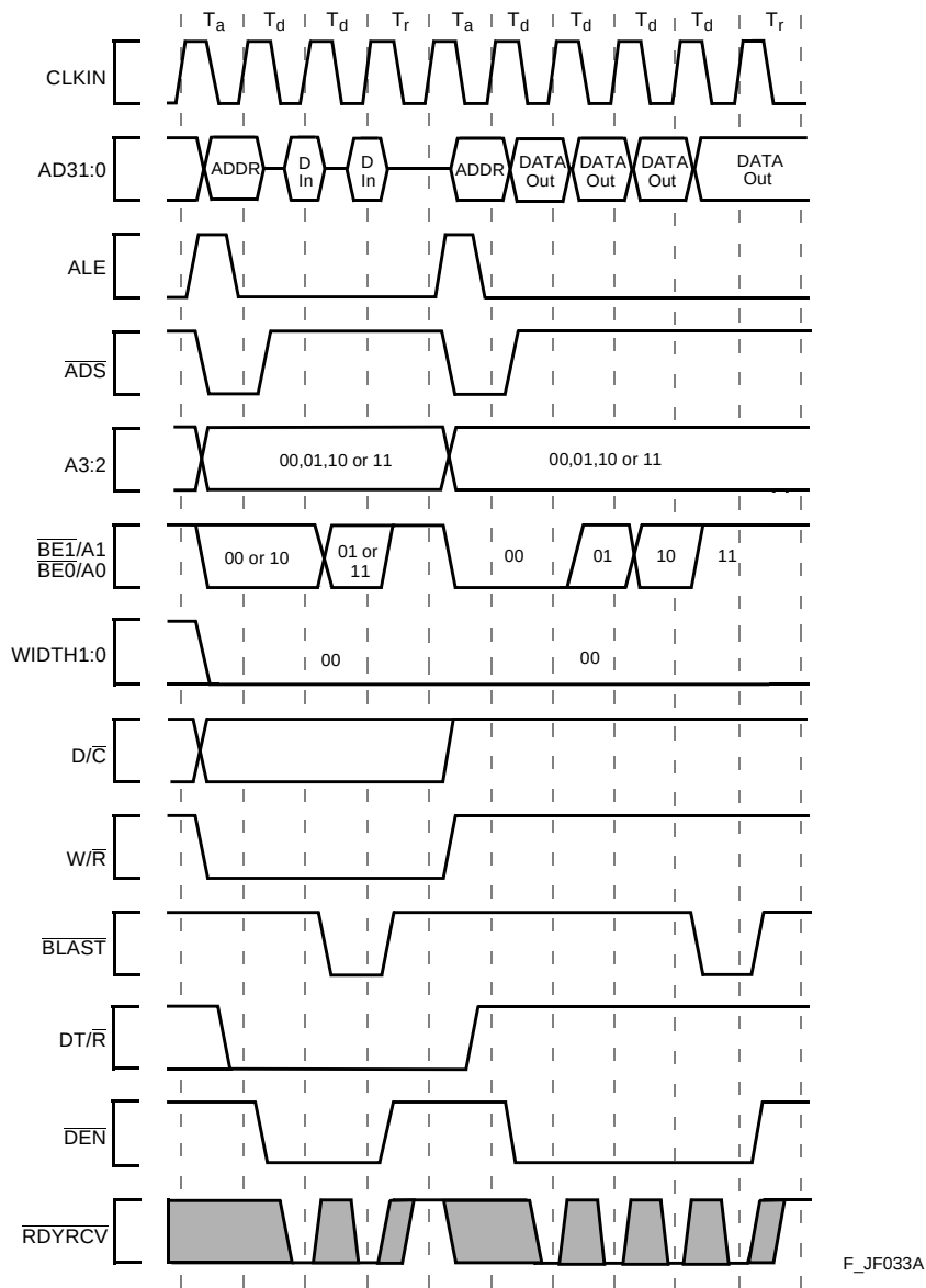
Figure 27. Burst Read and Write Transactions Without Wait States, 8-Bit Bus
