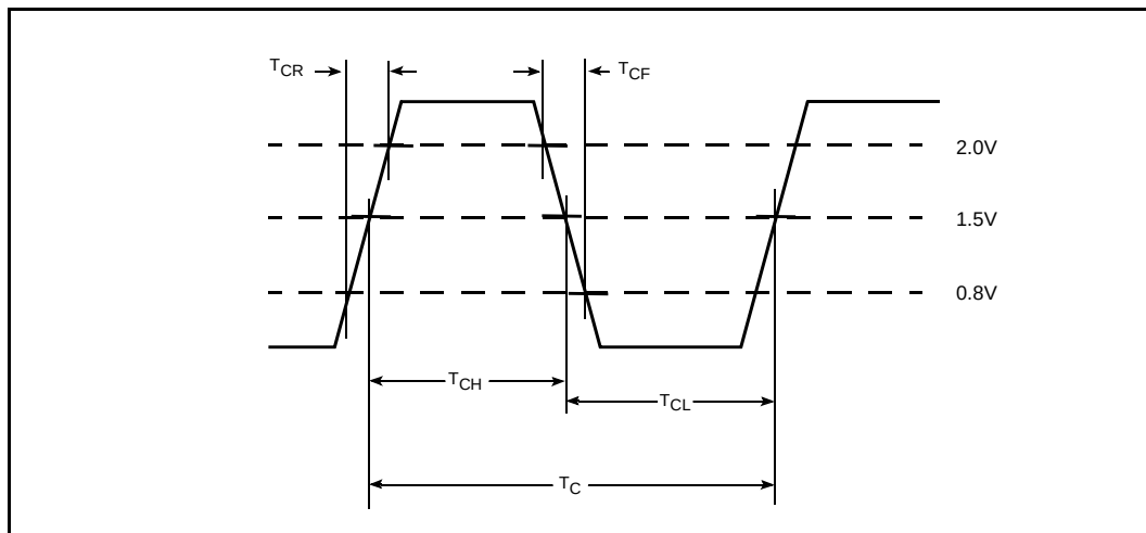
Figure 10. CLKIN Waveform
