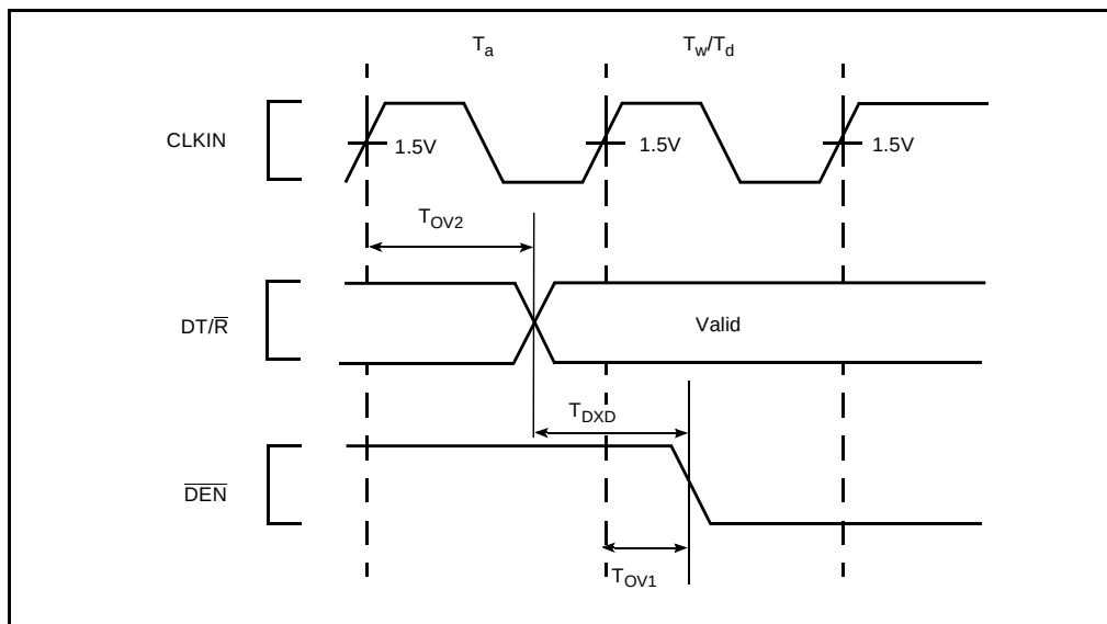
Figure 18. DT/R and \overline{\text{DEN}} Timings Waveform
