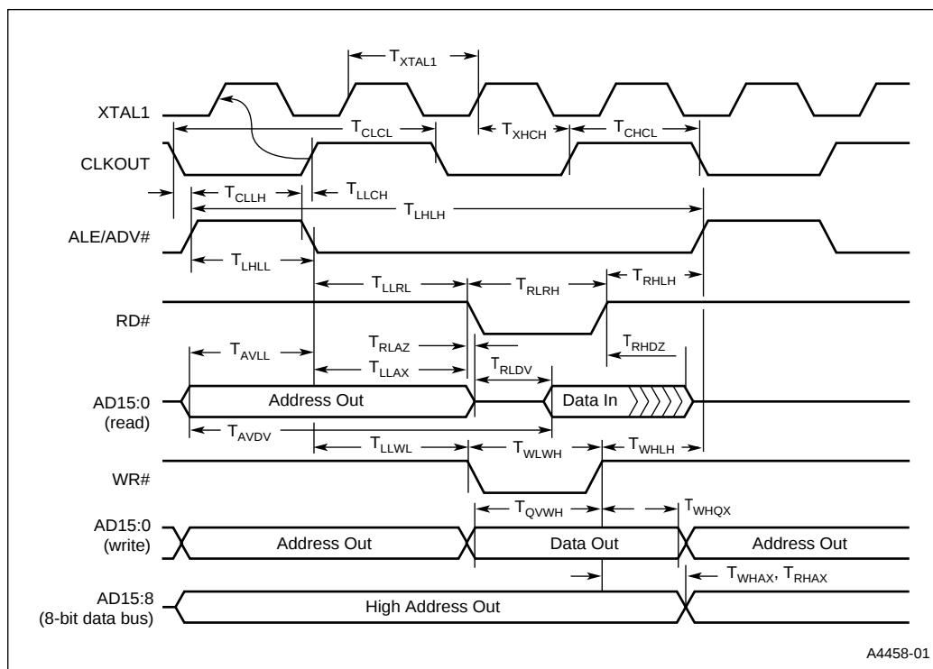
Figure 4. System Bus Timing
