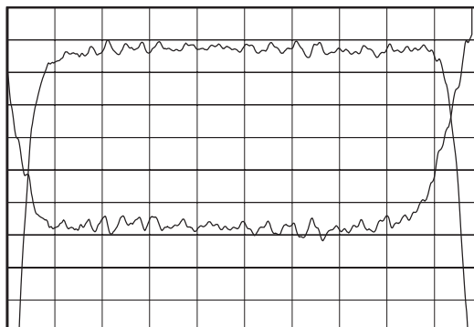
Horizontal: 2.5 MHz/Div Vertical: 1 dB/Div Vertical: 5 deg/Div
