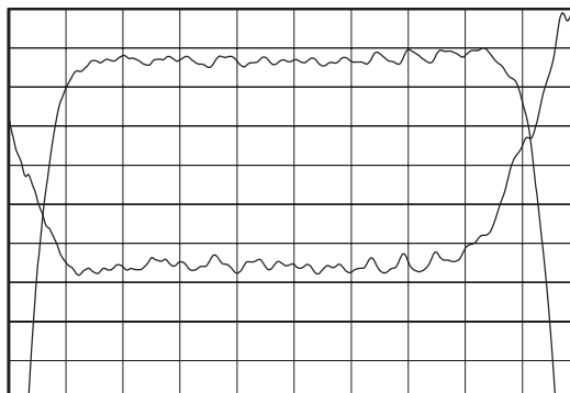
Horizontal: 1.7 MHz/Div Vertical: 1 dB/Div Vertical: 5 deg/Div
