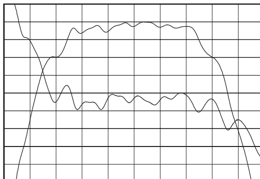
Horizontal: 500 kHz/Div Vertical: 1 dB/Div Vertical: 4 deg/Div
