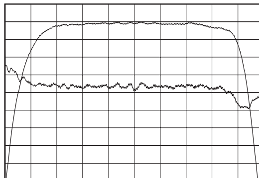
Horizontal: 4 MHz/Div Vertical: 1 dB/Div Vertical: 15 nsec/Div
