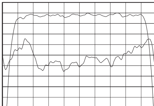
Horizontal: 650 kHz/Div Vertical: 1 dB/Div Vertical: 2 deg/Div
