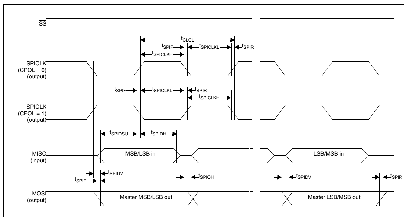
Figure 20: SPI Master timing (CPHA = 0)
