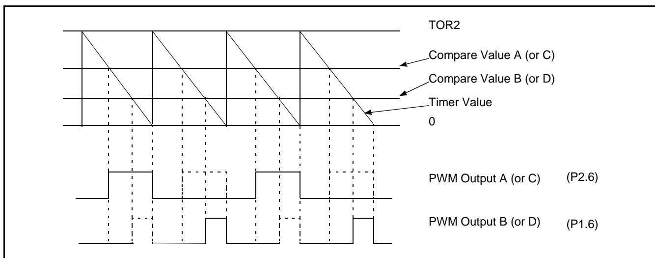
Figure 9: Alternate output mode
