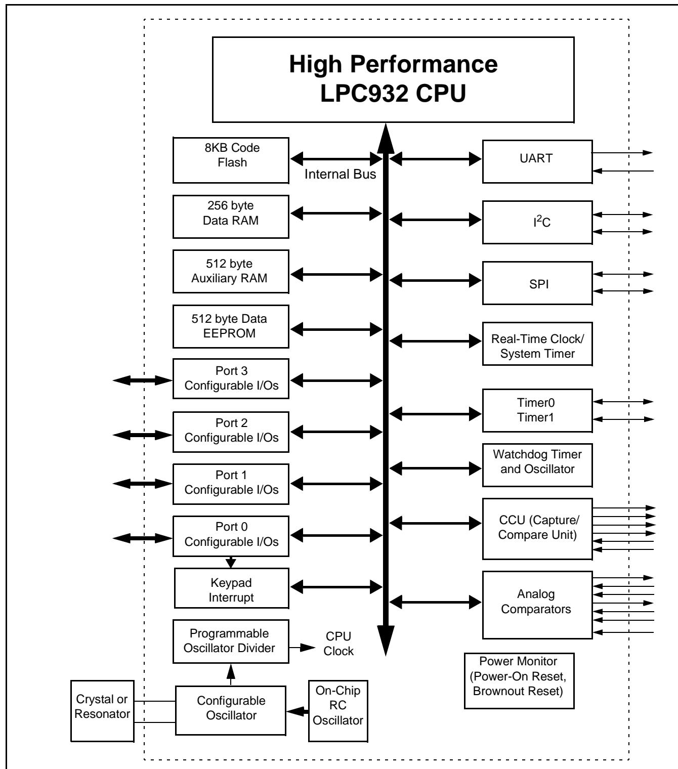
Figure 2: Block diagram.
