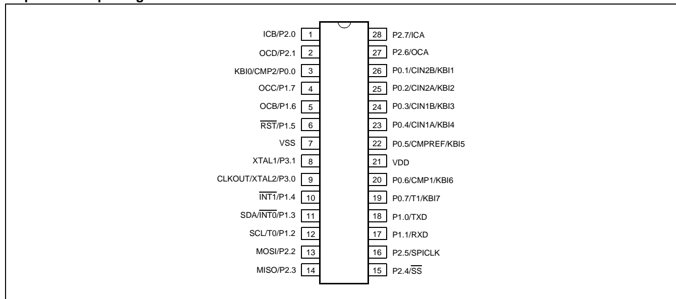
Figure 3: TSSOP28 pin configuration.
