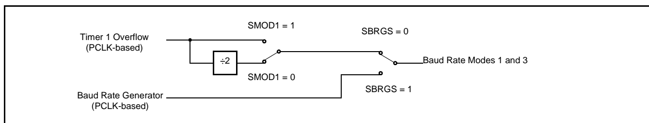
Figure 11: Baud rate sources for UART (Modes 1, 3)
