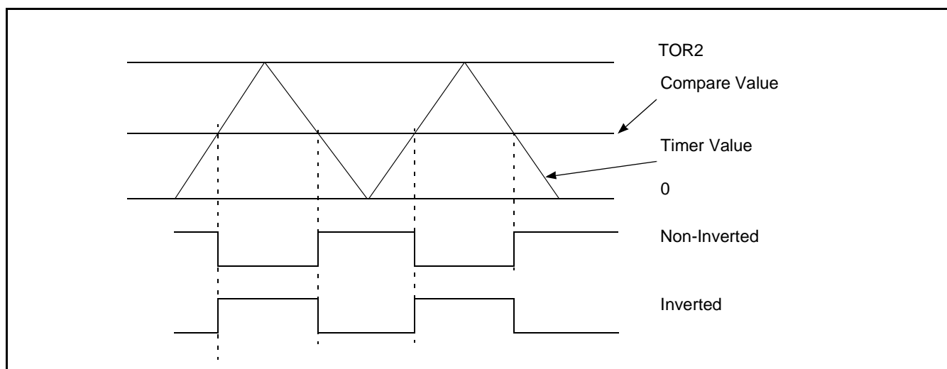
Figure 8: Symmetrical PWM
