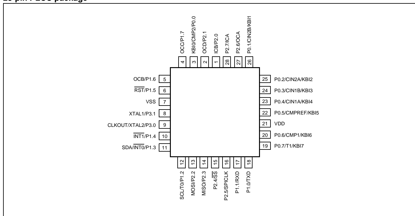
Figure 4: PLCC28 pin configuration.
