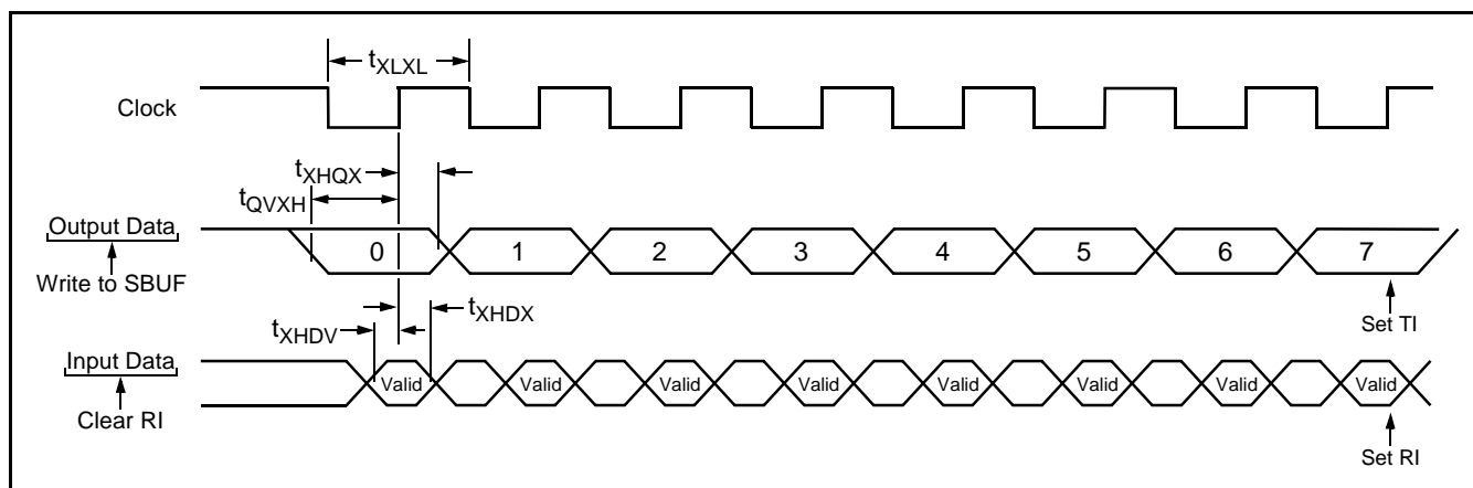
Figure 24: Shift Register Mode timing
