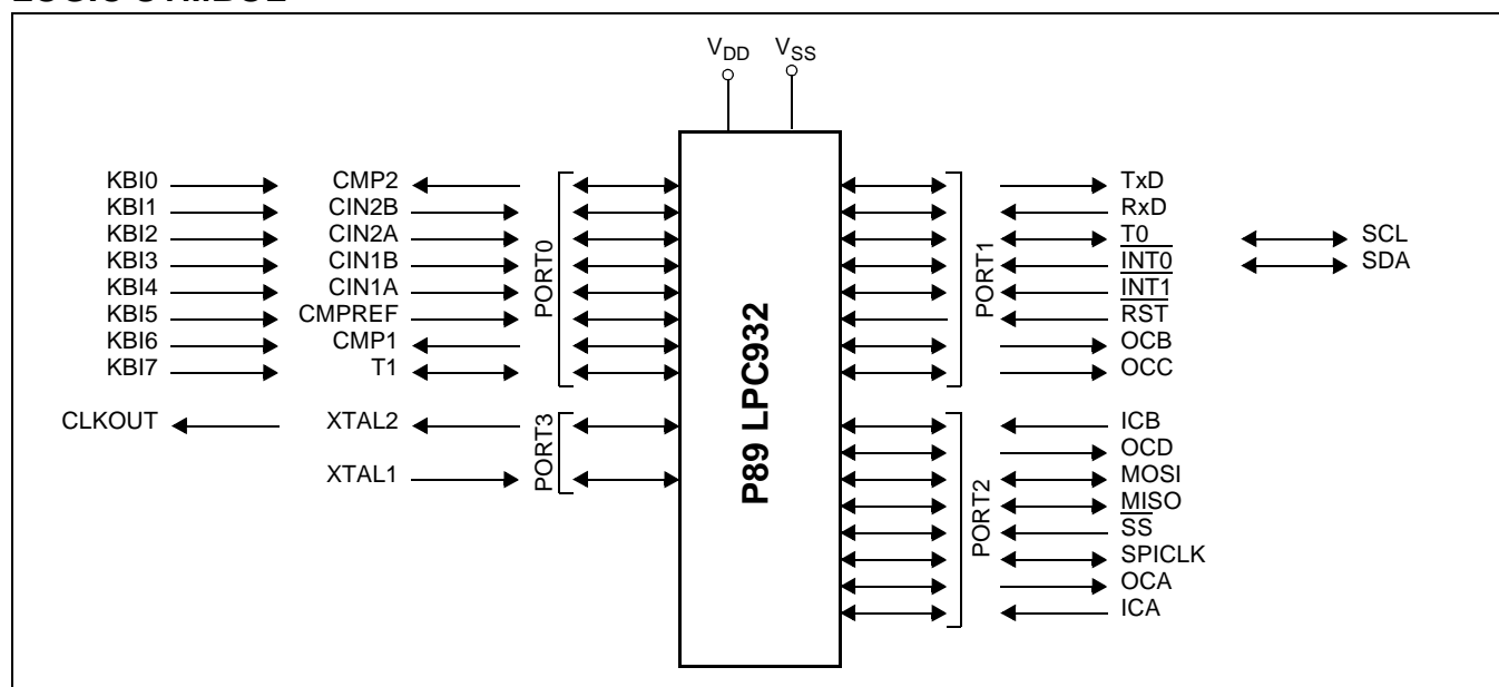
Figure 1: Logic symbol.
